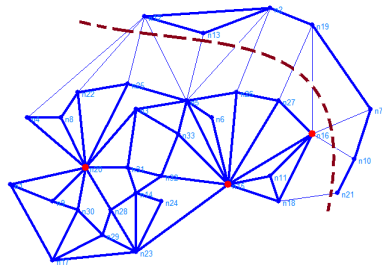
Figure 5: Best cut for 15 % budget
