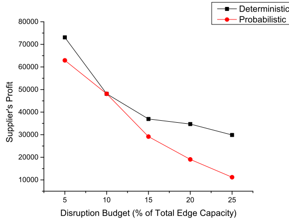
Figure 3: Comparison of deterministic and randomized algorithm for the test network
