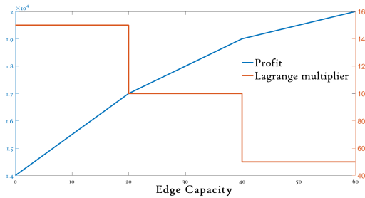
Figure 2: Illustration for proposition 1.
