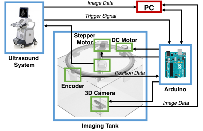
Fig. 3. System Diagram of ultrasound imaging system. An Arduino is used to control the stepper and DC motor, and to ensure that data collected from the 3D camera and encoder are synchronized with the ultrasound imaging system.
