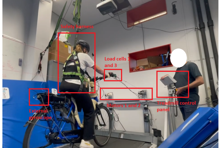
(a) Top view diagram of bicycle handlebar perturbation system. (b) A participant on the bicycle in the safety harness with the Bump'Em motor lines attached to the ends of the handlebars.
