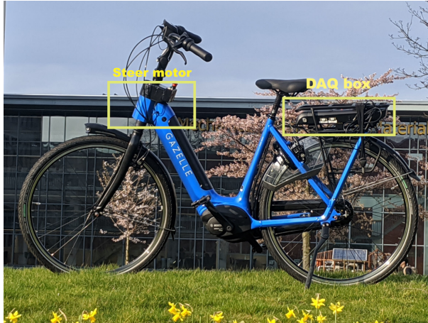
Figure 1: Balance assist bicycle prototype with electric motor in the steering column and data acquisition and control electronics mounted in the rear rack; first introduced in [5].
