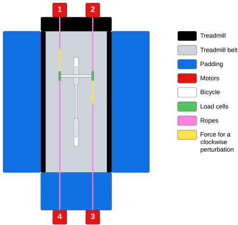
(a) Top view diagram of bicycle handlebar perturbation system. (b) A participant on the bicycle in the safety harness with the Bump'Em motor lines attached to the ends of the handlebars.
