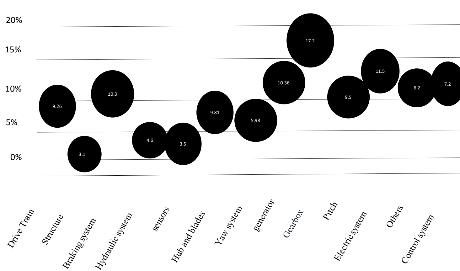
Figure. 2. Average component failure rate of wind turbines (WT)
