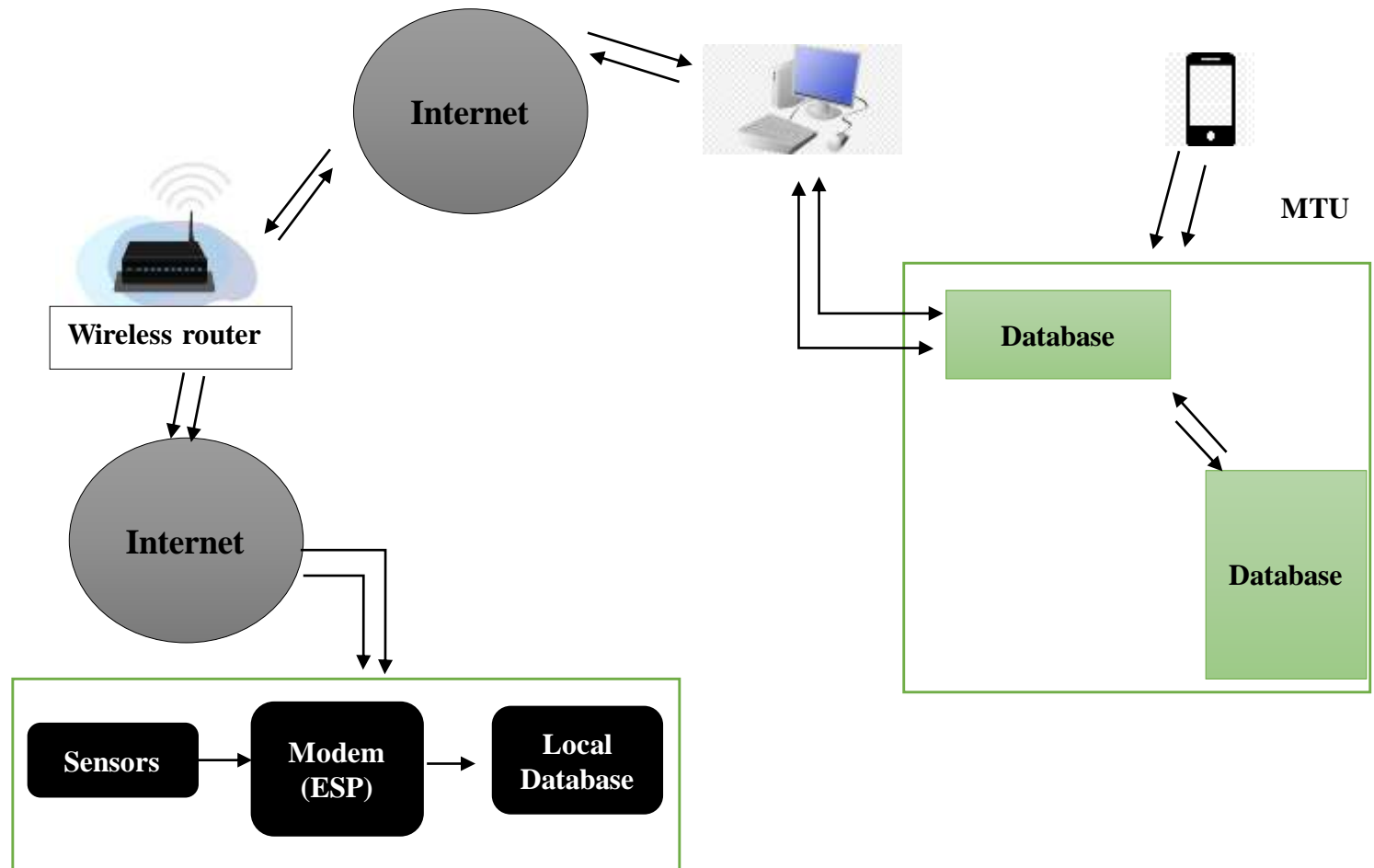
Figure. 7. Network topology of SCADA system
