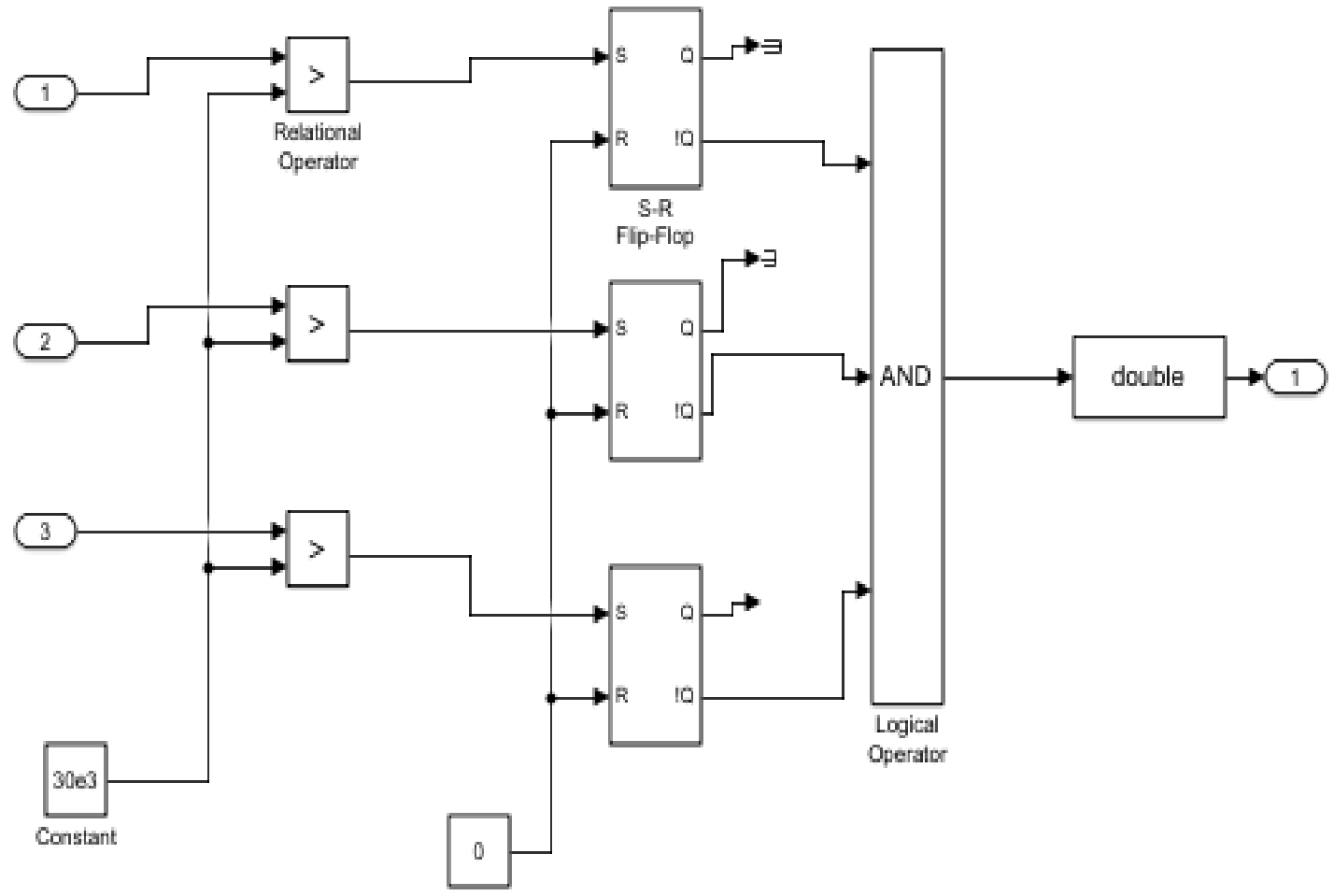
Figure. 7. Subsystem of three-phase fault relay
