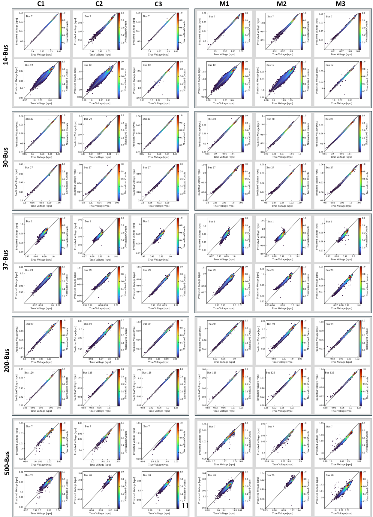
Figure 5: Comparison of true (from the external testset) and predicted voltage magnitude (vpv) for control models (C1, C2, C3) and candidate models (M1, M2, and M2), respectively. The bus nodes displayed were selected to show the worst-case predictions and hence the reason for the model selection decision. Similar plots for all buses (and models) are available as supplementary datasets.
