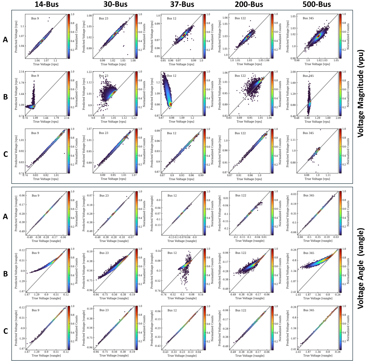
Figure 8: Comparison of true vs. predicted voltage magnitudes (upper panel) and angles (lower panel) to highlight the benefits of PowerModel-AI's on-the-fly learning capability. In each panel, row A shows the base model's performance on an external test set from the \Delta_{\max}^* domain, while rows B and C present the performance of the base and updated models on a new test set from the \Delta_{\max} domain, as outlined in Table 1. The nodes in the plots are selected based on the base model's best predictions for the \Delta_{\max} domain (Row B).
