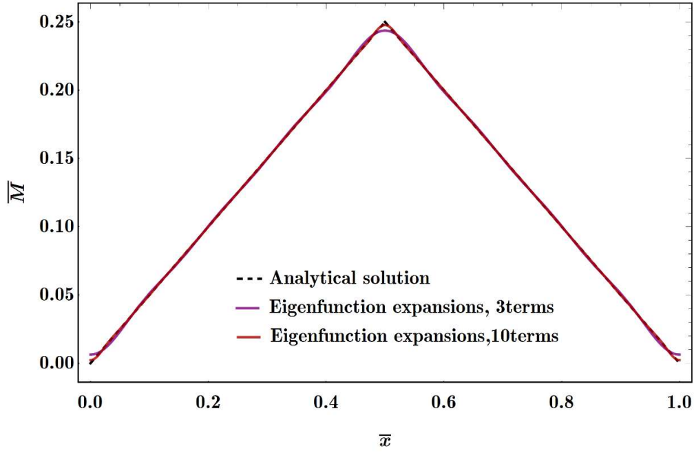
Fig. 3. Flexural moment of a simply supported nanobeam subject to a transverse force at the midspan, analytical solution vs. eigenfunction expansion
