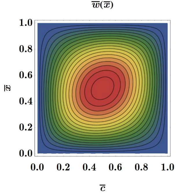
Fig. 11. Contour plot of the flexure of the mixture unified gradient beam with simple supports subject to a transverse force at \overline{c} for prescribed parameter \alpha = 1/5, \zeta = 1/4, \eta = 1/3
