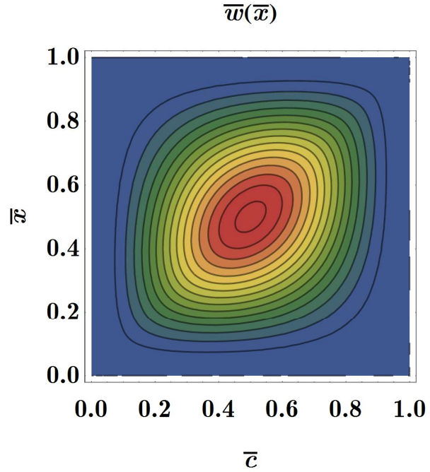
Fig. 12. Contour plot of the flexure of the mixture unified gradient beam with fixed-ends subject to a transverse force at \overline{c} for prescribed parameter \alpha = 1/5, \zeta = 1/4, \eta = 1/3
