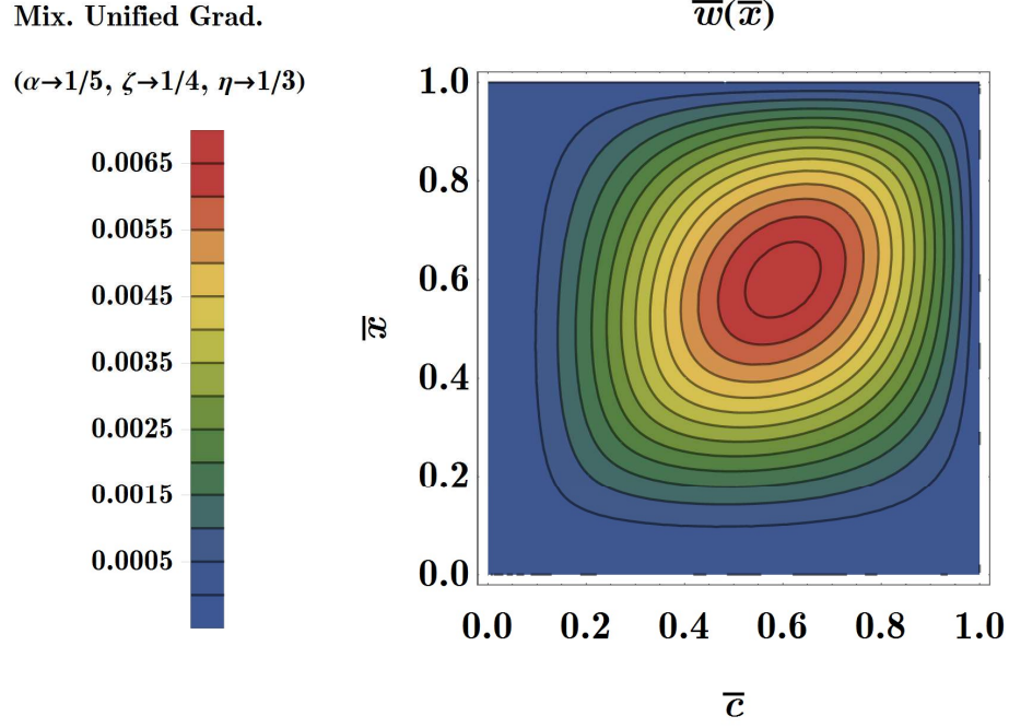
Fig. 13. Contour plot of the flexure of the mixture unified gradient beam with fixed-simple ends subject to a transverse force at \overline{c} for prescribed parameter \alpha = 1/5, \zeta = 1/4, \eta = 1/3
