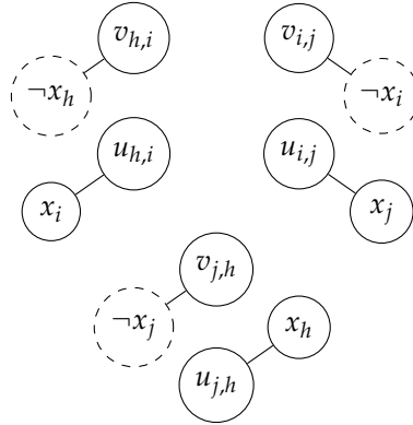
Figure 1. variable gadget for the occurrences of x in clauses c_h, c_i, c_j of \phi .
