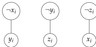
Figure 3. clause gadget corresponding to the clause c_i = (x \vee y \vee z) in \phi .
