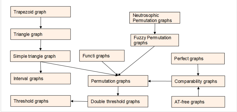
Fig. 6. Permutation Graphs Hierarchy. The graph class at the origin of an arrow contains the graph class at the destination of the arrow.
