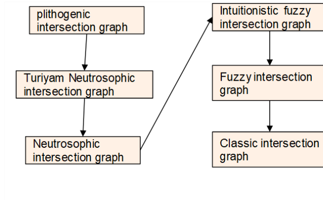
Fig. 15. Uncertain Intersection graphs Hierarchy. The graph class at the origin of an arrow contains the graph class at the destination of the arrow.
