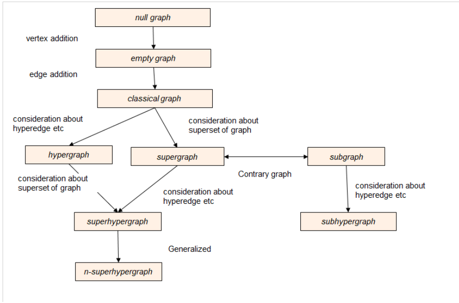
Fig. 2. HyperGraph Hierarchy
