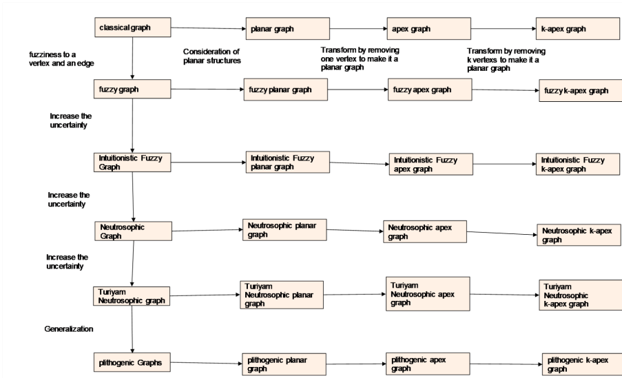
Fig. 1. Graph Hierarchy in this paper
