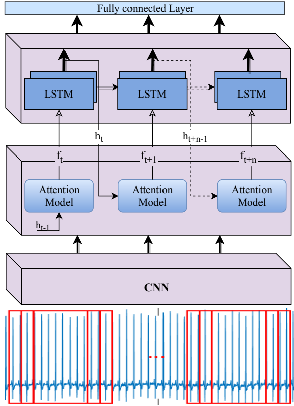
Figure 2: The network architecture of attention model.
