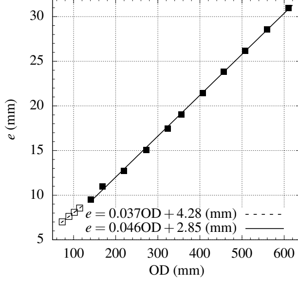
Figure 1: Example of a typical linear dependence of the pipe thickness with the outside diameter ( OD = D + 2e ). Here, OD and thickness values correspond to SCH 80 pipelines following Christensen et al. (2004) .
