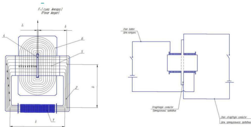
Fig.1 - Schematic diagram of a power electromagnetic device with a configuration of magnetic fields.
