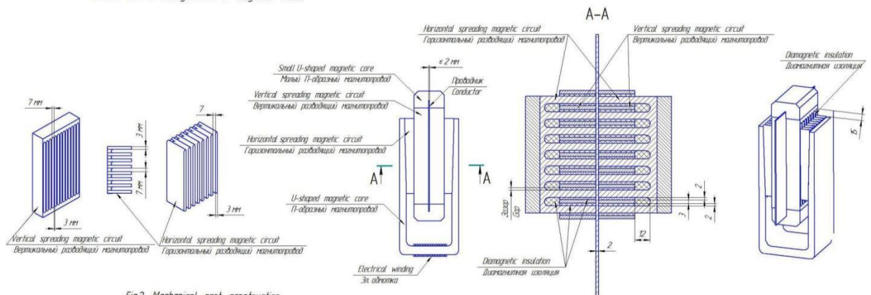
Fig.2. Mechanical part construction
