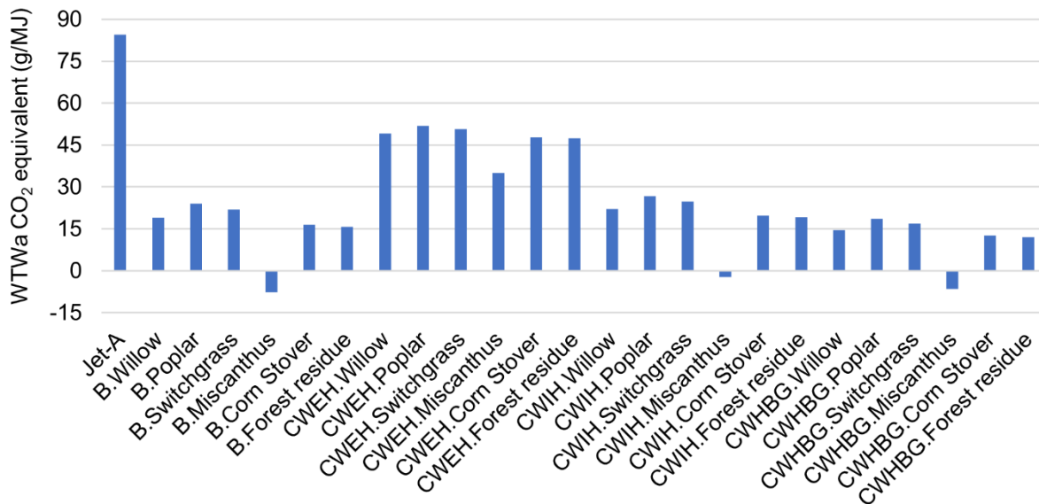
Figure 8.6. WTWa CO 2 equivalent emission comparison of different STJ feedstocks for 2020 (with only CO 2 emissions in PTWa phase)
