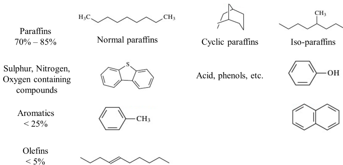
Figure B.12. Composition of the conventional jet fuel (information source [375])
