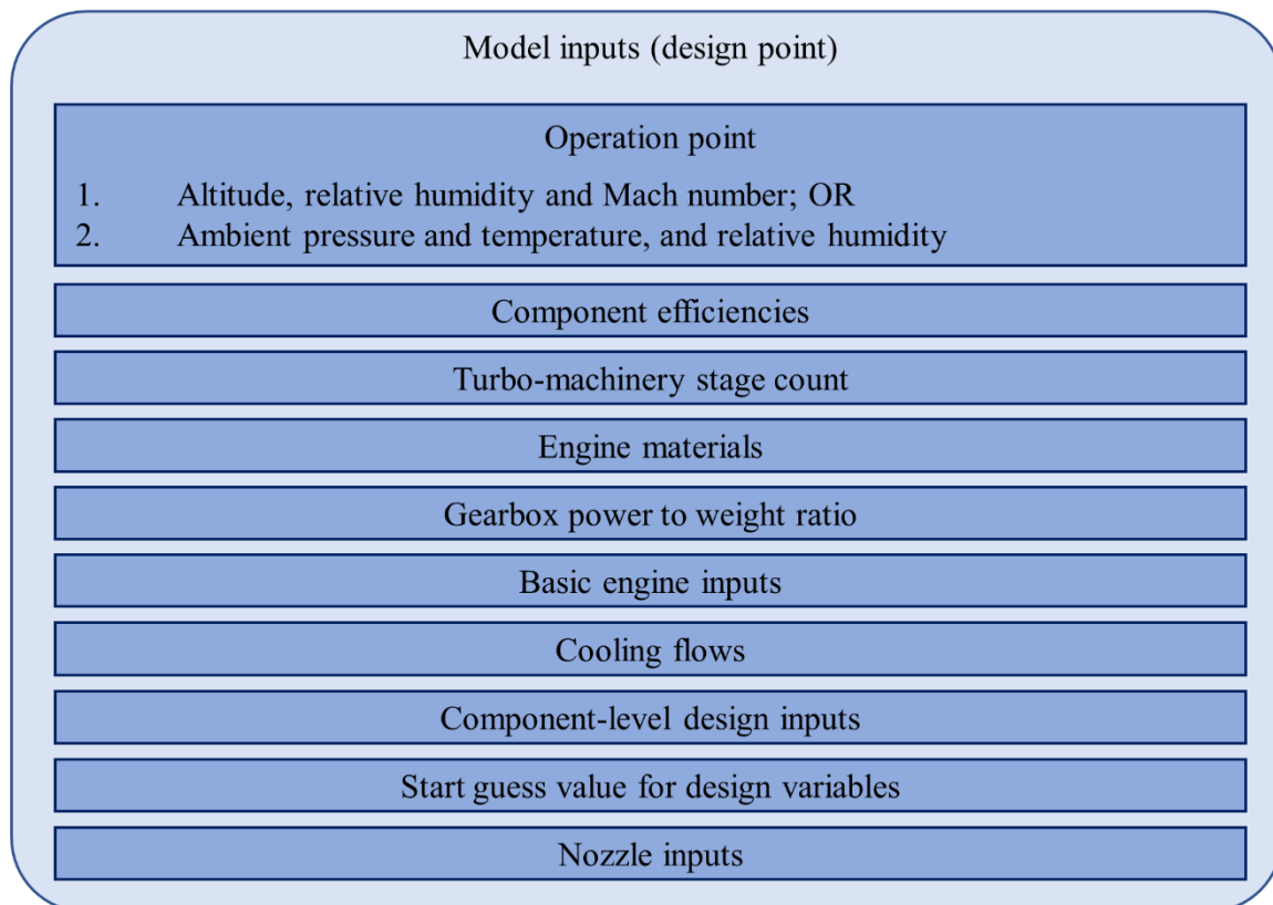
Figure 6.8. Engine model inputs
