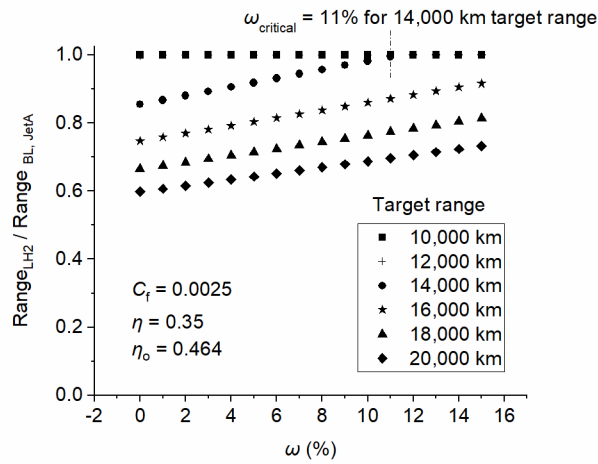
Figure B.2. Effect of design target range on \omega_{\text{critical}} of the LH 2 aircraft
