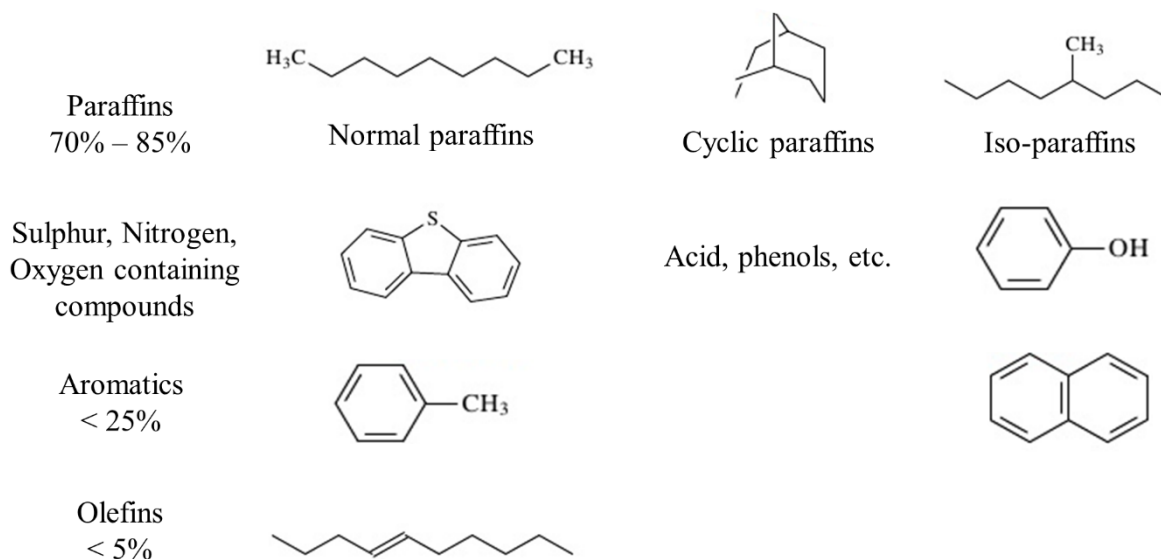
Figure B.12. Composition of the conventional jet fuel (information source [365])
