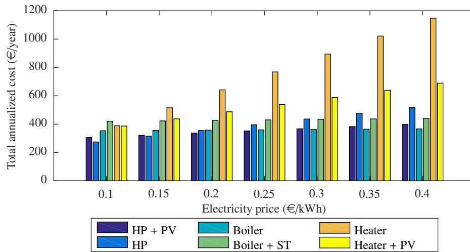
Figure 9: Influence of the electricity price on the total cost.
