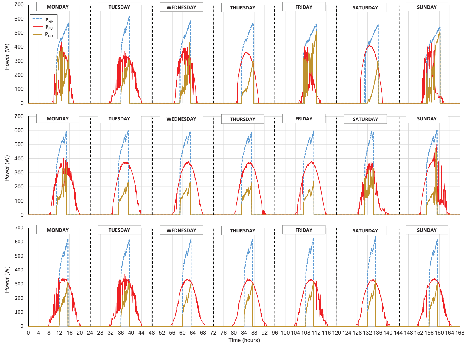
Figure 4: Electricity production and consumption during one week of January (top), April (middle) and June (bottom).
