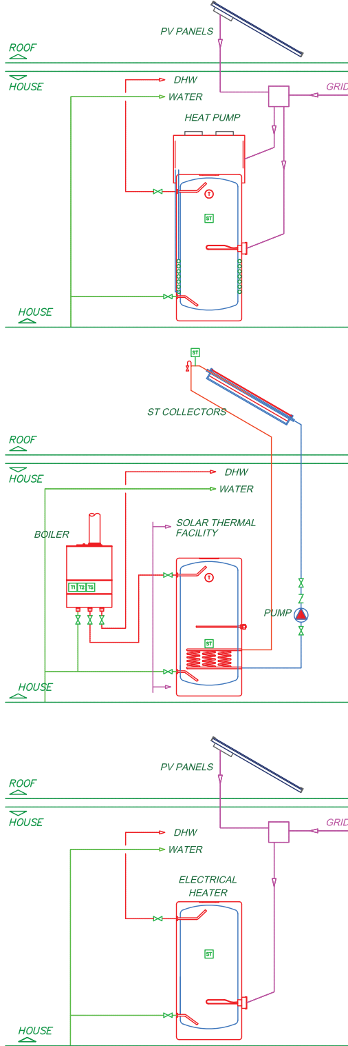
Figure 6: Sketch of the facilities of the comparison which use solar energy. Top: HP + PV. Middle: Boiler + ST. Bottom: Heater + PV
