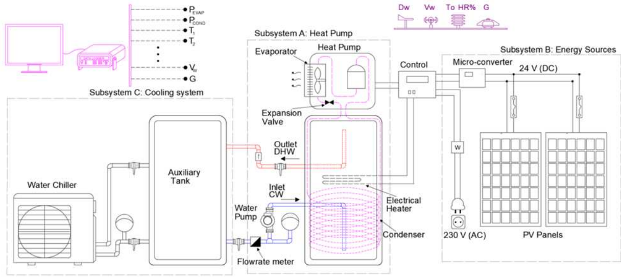
Figure 3: Experimental facility.
