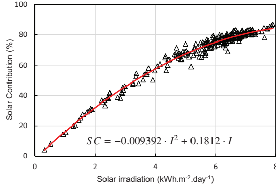
Figure 5: Solar contribution to the heat pump consumption ( HP+PV system) as a function of the irradiation on the surface of the PV panels ( 45^\circ ). Correlation in red: .
