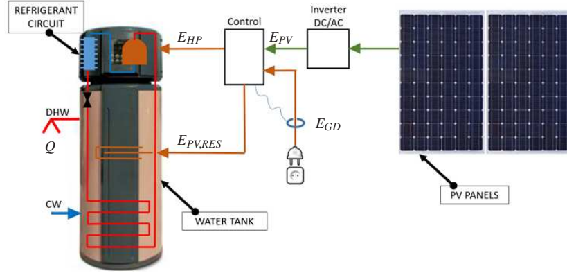
Figure 1: Sketch of photovoltaic assisted heat pump for domestic hot water production (HP+PV system).
