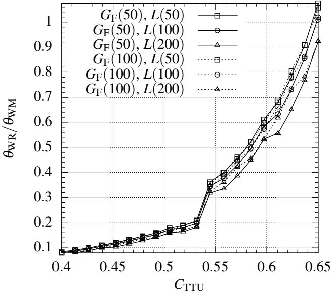
Figure 15: Ratio between recirculation and makeup components of the water unit cost, as a function of the thickener underflow concentration. In the legend, values in brackets correspond to thousand tonnes per day for G_F and pipeline length in kilometers in the case of the variable L .
