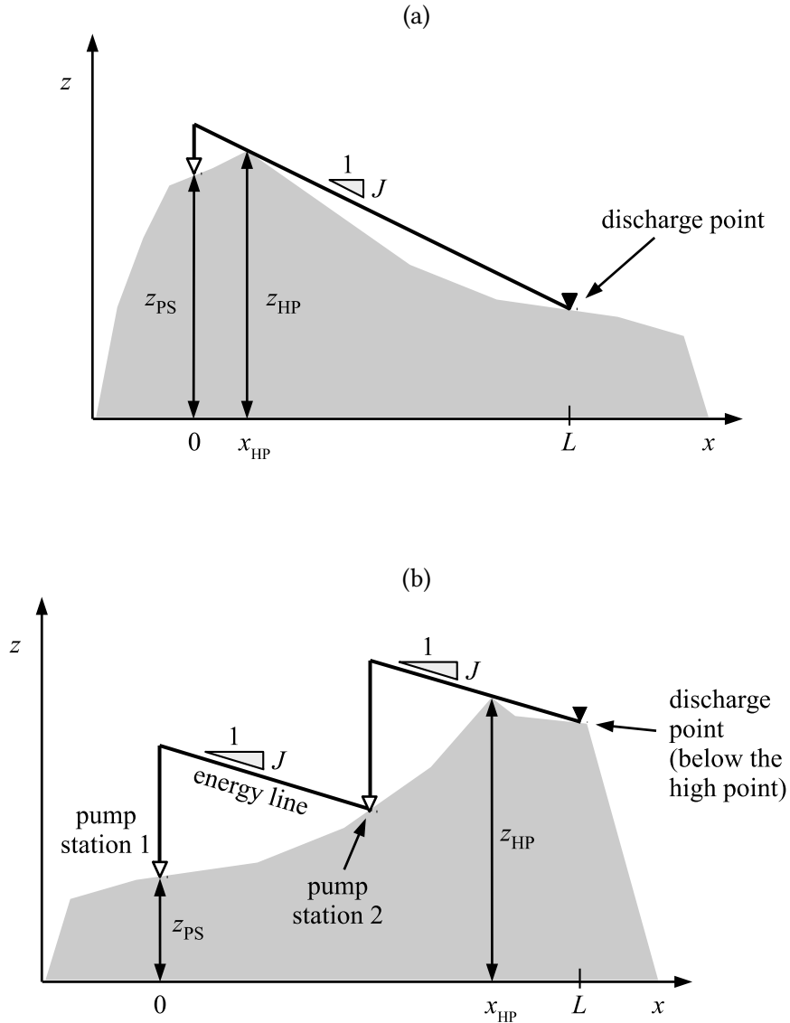
Figure 10: Schematic of the topography and energy components considered in the specific energy calculation for single diameter pipeline with the energy line with virtually zero relative pressure at the high point, located at x_{HP} = \lambda_{HP}L . (a) Ore concentrate pipeline, (b) Water pipeline. In (b), the facility has been shown with two pump stations. This has no influence on the specific energy analysis result during steady state when all the pipeline segments have constant diameter.
