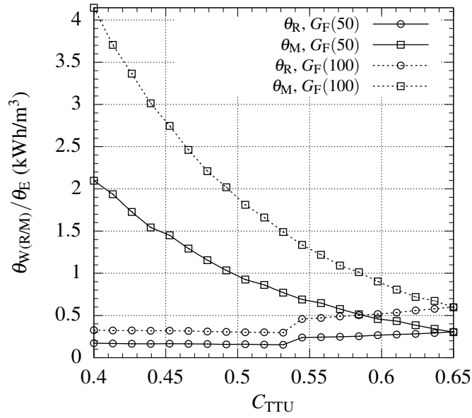
Figure 13: Components of the ratio between water and energy unit costs in terms of the thickener underflow concentration, C_{TTU} , for fixed values of the pipeline length and the fraction of water recovered from the TSF of L = 100 km and \lambda_{TDR} = 0.5 , respectively. In the legend, values in brackets correspond to thousand tonnes per day for G_F .
