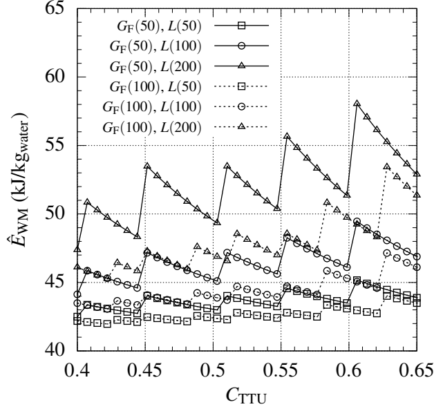
Figure 7: Specific energy component related to water makeup ( \hat{E}_{WM} ), in terms of the thickener underflow concentration, C_{TTU} , with Y = 0.025 . In the legend, values in brackets correspond to thousand tonnes per day for G_F and pipeline length in kilometers in the case of the variable L .
