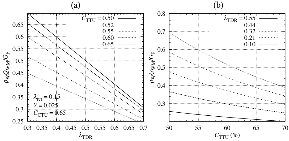
Figure 3: Makeup water mass flow normalized by plant throughput for \lambda_{ret} = 15\% , Y = 2.5\% , C_{CTU} = 65\% . (a) As a function of the fraction of water recovery from the TSF and (b) in terms of tailings thickener underflow concentration.
