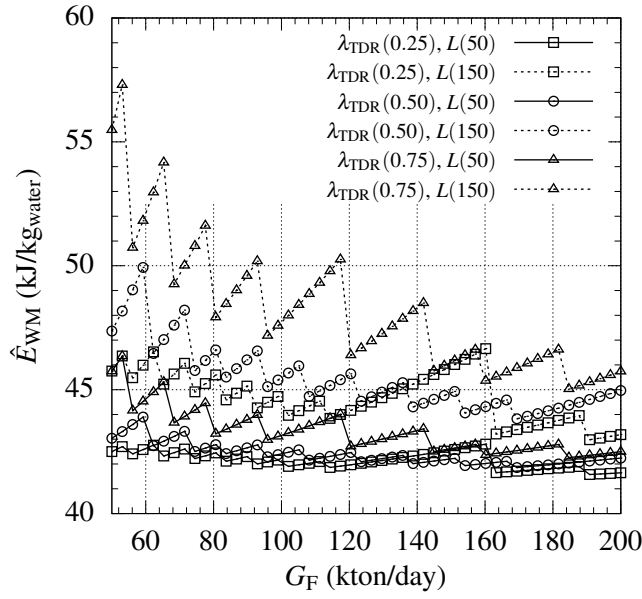
Figure 8: Specific energy component related to water makeup ( \hat{E}_{WM} ), in terms of the plant feed throughput, G_F , with Y = 0.025 . In the legend, values in brackets correspond recovery fraction from the TSF ( \lambda_{TDR} ) and pipeline length in kilometers in the case of the variable L .
