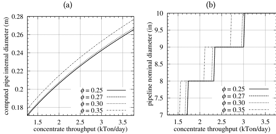
Figure 5: Pipeline diameter determination for ore concentrate using (a) a continuous approach and (b) the choice of the closest commercial available value, for different slurry volume fractions. In the present nomenclature, the x -axis corresponds to the concentrate throughput, equal to YG_F . Present values of the volume solids fraction of the concentrate are similar to those in real concentrate pipelines (Betinol and Jaime, 2004; Ihle and Tamburrino, 2012). Ore concentrate reference throughput values are on the order of those reported for large scale Chilean mining operations (Consejo Minero, 2002).
