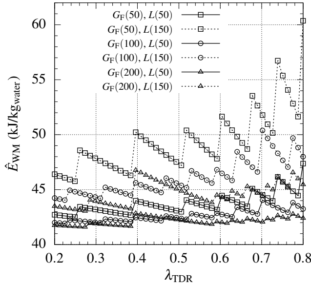
Figure 9: Specific energy component related to water makeup ( \hat{E}_{WM} ), in terms of the fraction of water recovery from the TSF, \lambda_{TDR} , with Y = 0.025 . In the legend, values in brackets correspond to thousand tonnes per day for G_F and pipeline length in kilometers in the case of the variable L .
