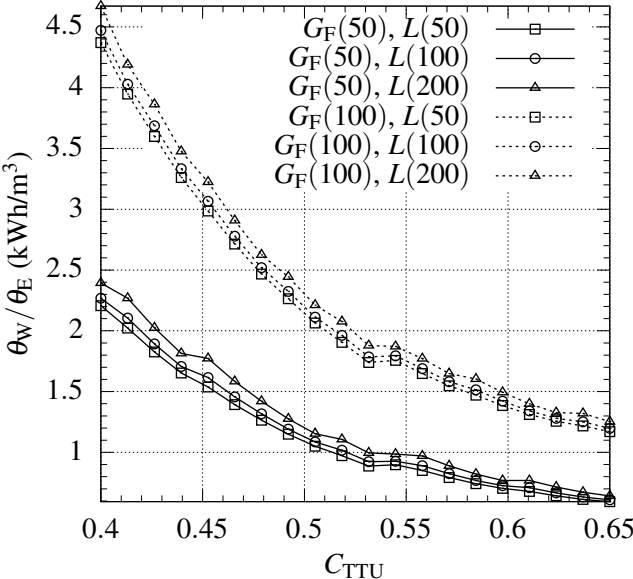
Figure 12: Ratio between water and energy unit costs in terms of the thickener underflow concentration. In the legend, values in brackets correspond to thousand tonnes per day for G_F and pipeline length in kilometers in the case of the variable L .
