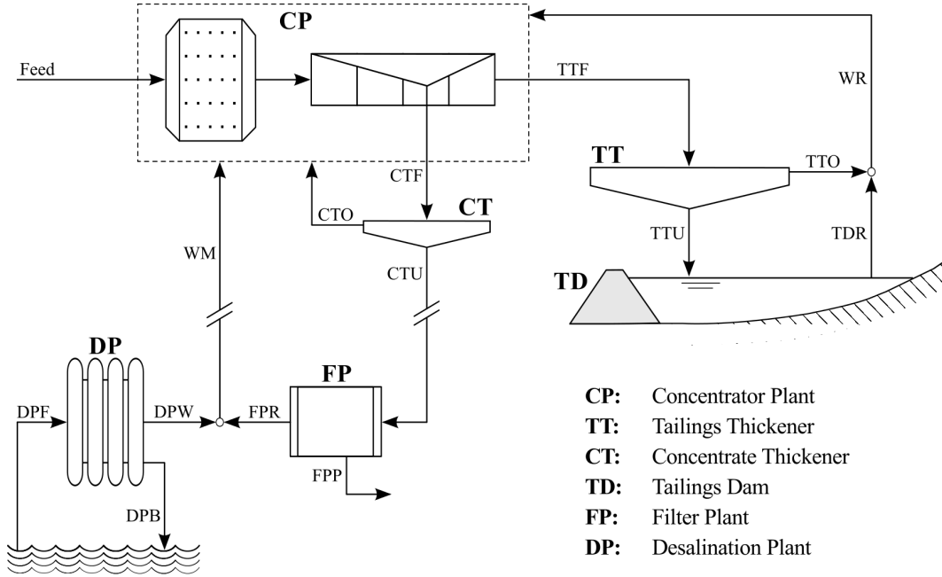
Figure 2: Schematic of the flows at the TSF. It is noted that both solid and liquid accumulation occurs.
