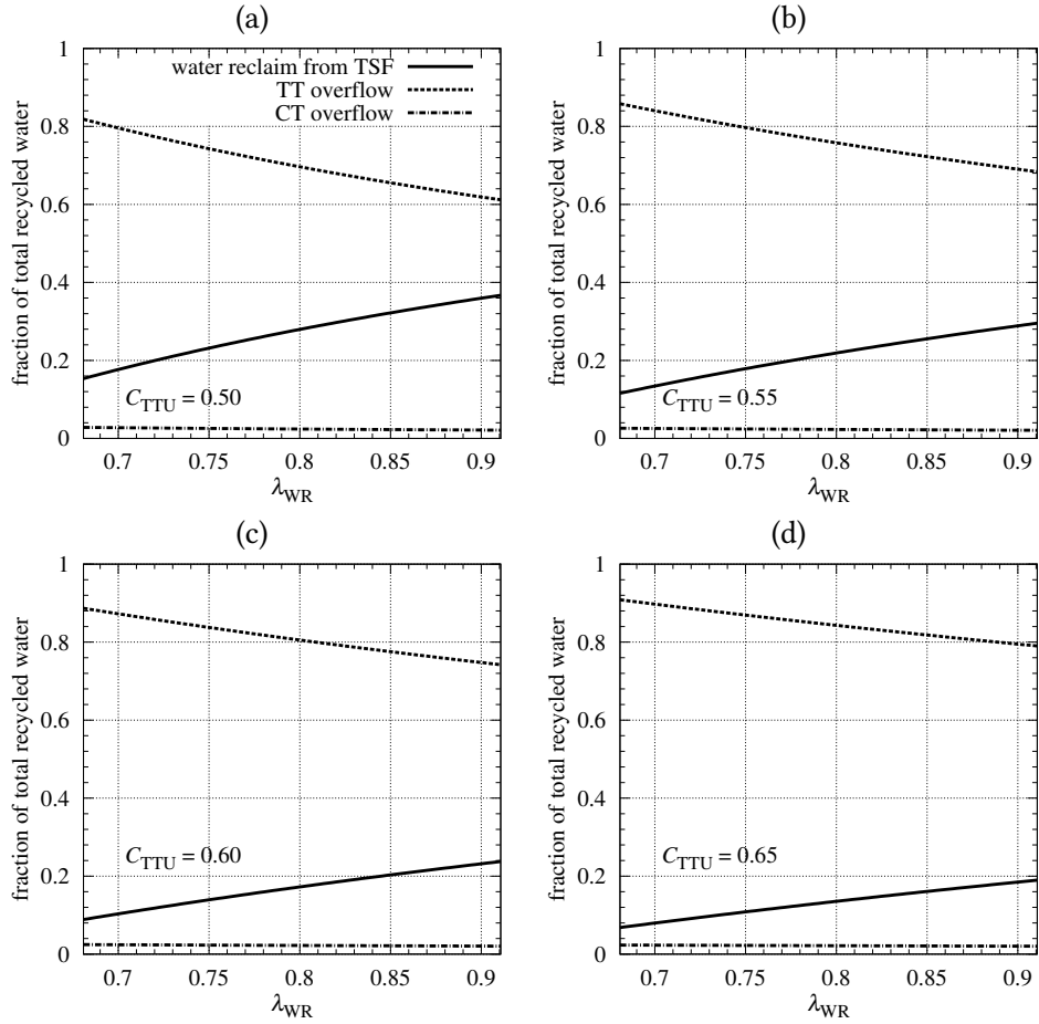
Figure 4: Relative fractions of the total water recirculation, corresponding to water reclaimed from the TSF, water recycled from the concentrate and tailing thickeners (acronyms CT and TT, respectively), for (a) C_{TTU} = 50\% , (b) C_{TTU} = 55\% , (c) C_{TTU} = 60\% and (d) C_{TTU} = 65\% . Here, \lambda_{WR} is the fraction of the total flow which is recirculated in the plant.
