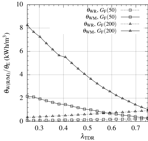
Figure 14: Components of the ratio between water and energy unit costs in terms of the fraction of water recovered from the TSF, \lambda_{TDR} , for fixed values of the pipeline length and the thickener underflow concentration of L = 100 km and C_{TTU} = 0.55 , respectively. In the legend, values in brackets correspond to thousand tonnes per day for G_F .
