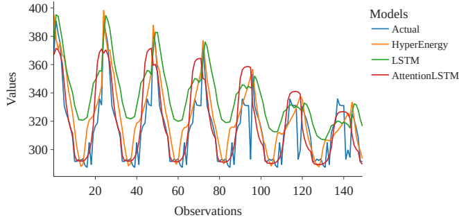
Fig. 4. Student Residence 1: actual versus the predicted value for top four models— HyperEnergy, LSTM, AttentionLSTM, and XGBoost.
