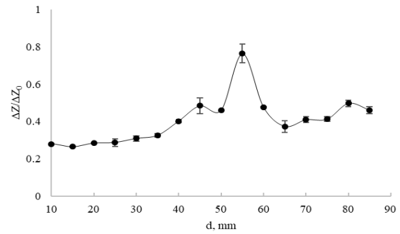
(b) Normalized impedance, E = 10 J
