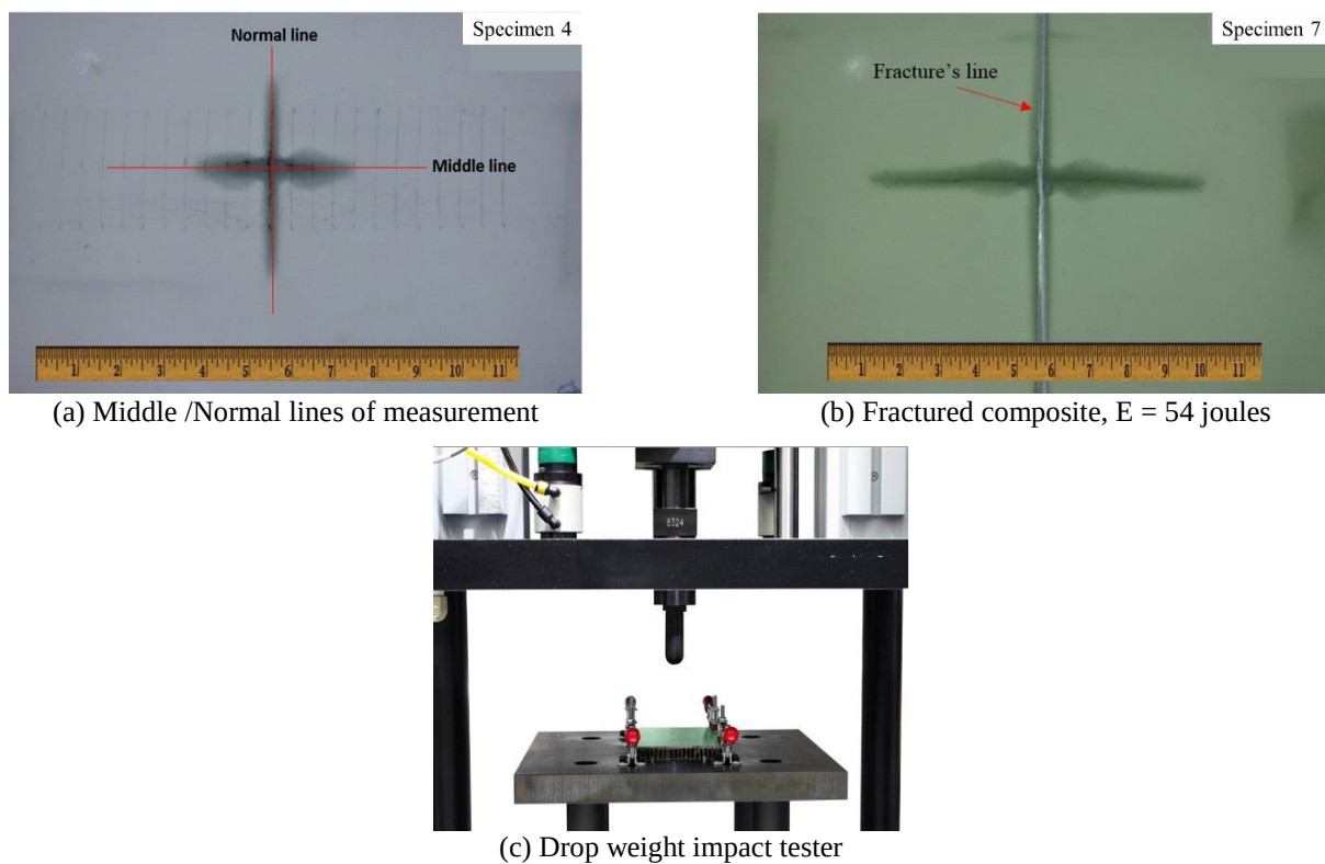
Fig. 6 Impact test and measurement setup
