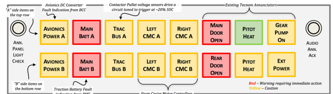
Fig. 5. The X-57 annunciator panel with electric propulsion indication.
