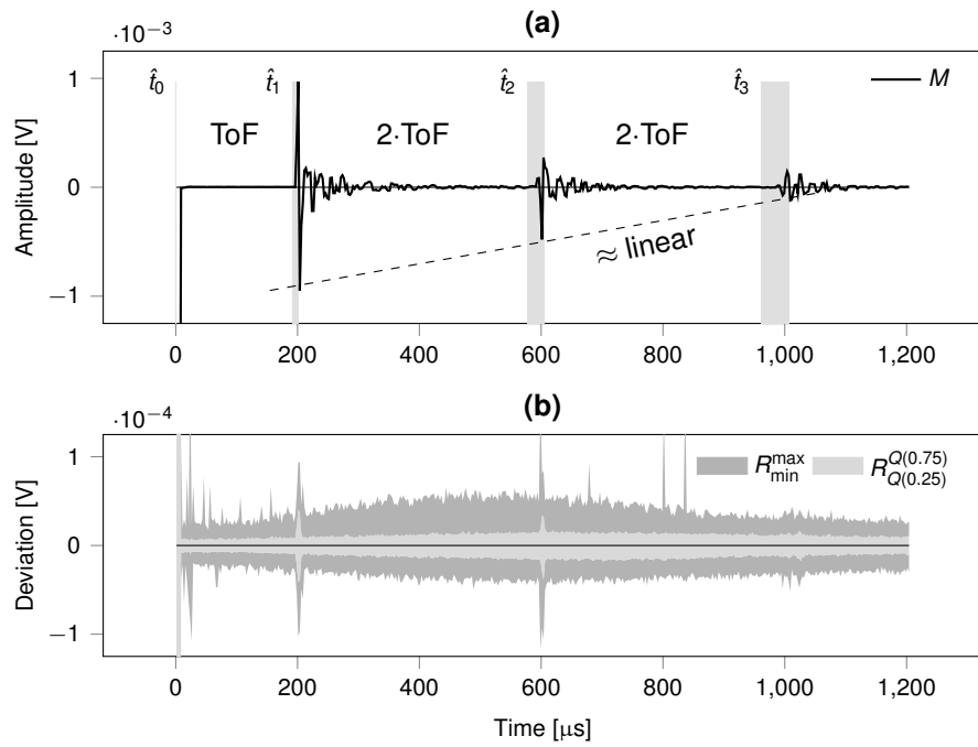
Figure 9: Test series 5, reference tests on air – primary wave, D = 70 mm. (a) Ensemble average M . (b) Deviation from ensemble average R .
