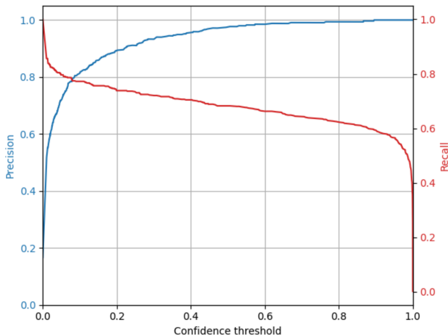
Fig 2. Precision vs. threshold results for BirdNET on the full dataset.
