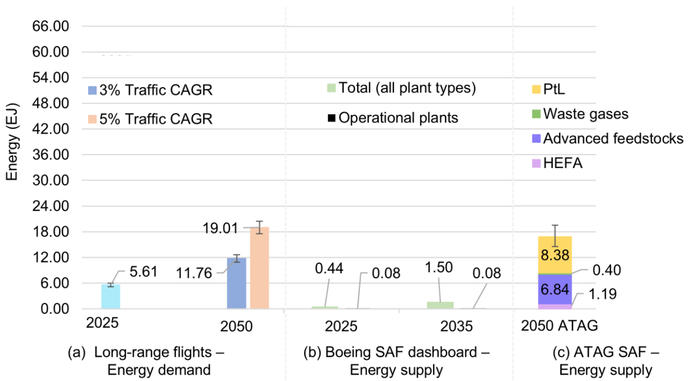
Figure 9. Energy demand forecast for long-haul aviation and supply of SAF
