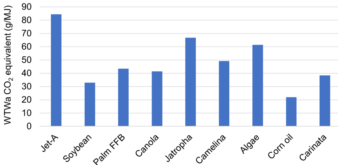
Figure 4. WTWa CO 2 equivalent emission comparison of different HEFA feedstocks for 2020 (with only CO 2 emissions in PTWa phase)
