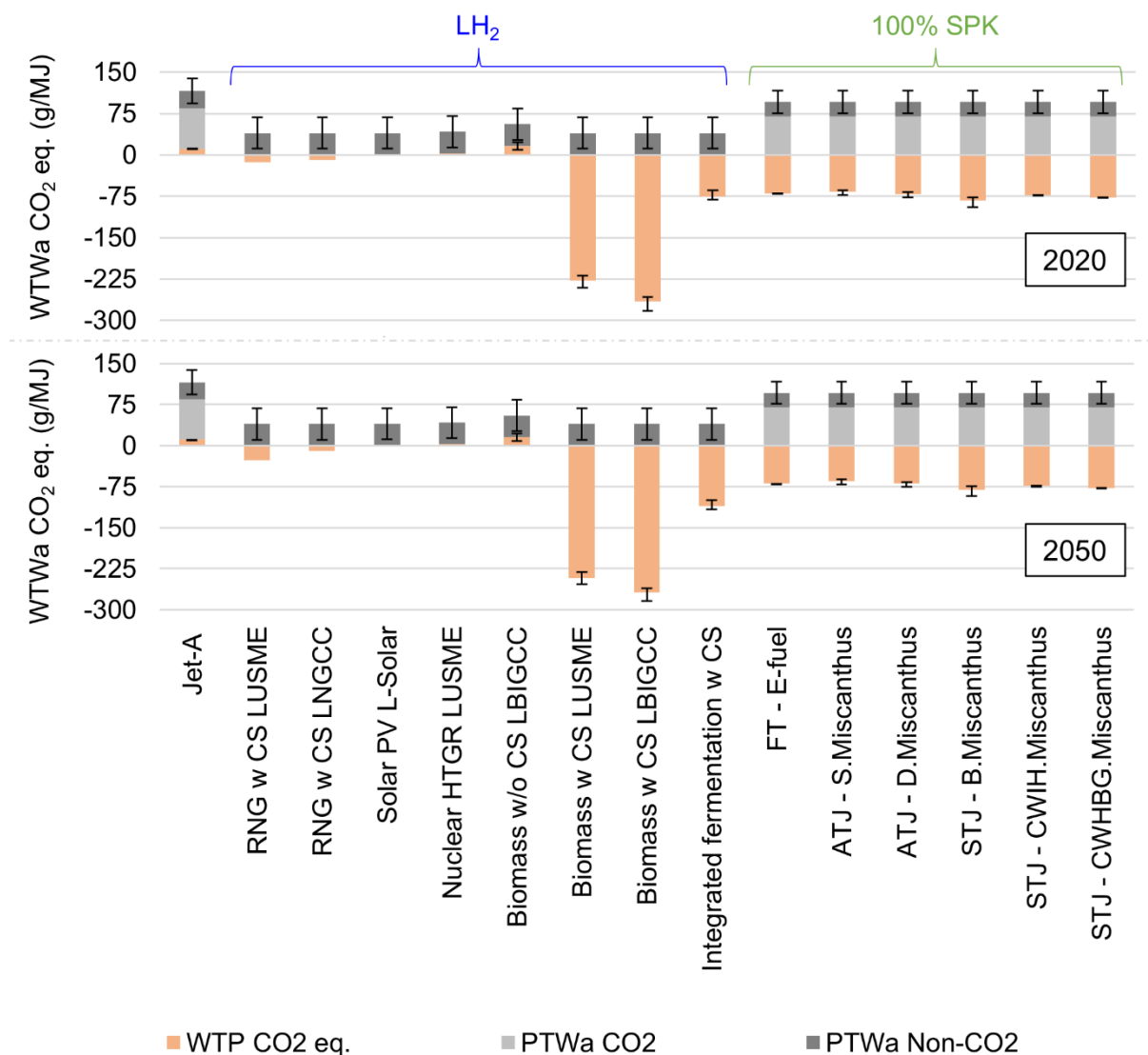
Figure 8. WTWa CO 2 equivalent emission comparison for different LH 2 and 100% SPK feedstock and pathways for 2020 and 2050 US energy mix scenarios including non-CO 2 effects
