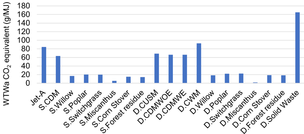
Figure 5. WTWa CO 2 equivalent emission comparison of different ATJ feedstocks for 2020 (with only CO 2 emissions in PTWa phase)
