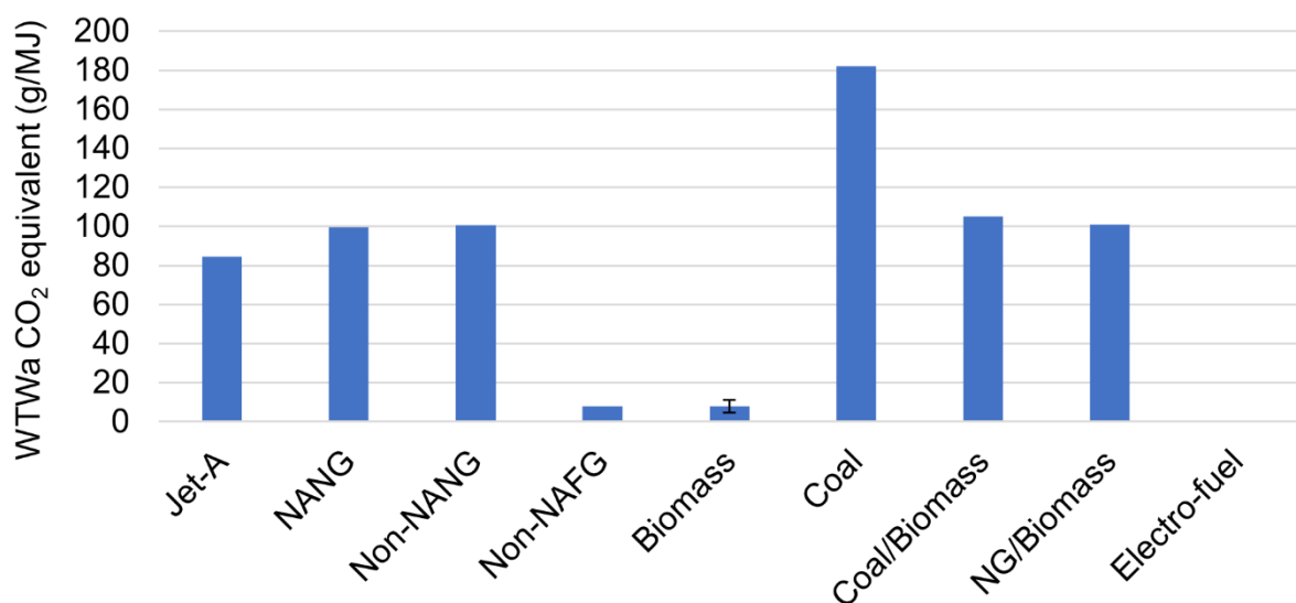
Figure 3. WTWa CO 2 equivalent emission comparison of different FT feedstocks for 2020 (with only CO 2 emissions in PTWa phase)
