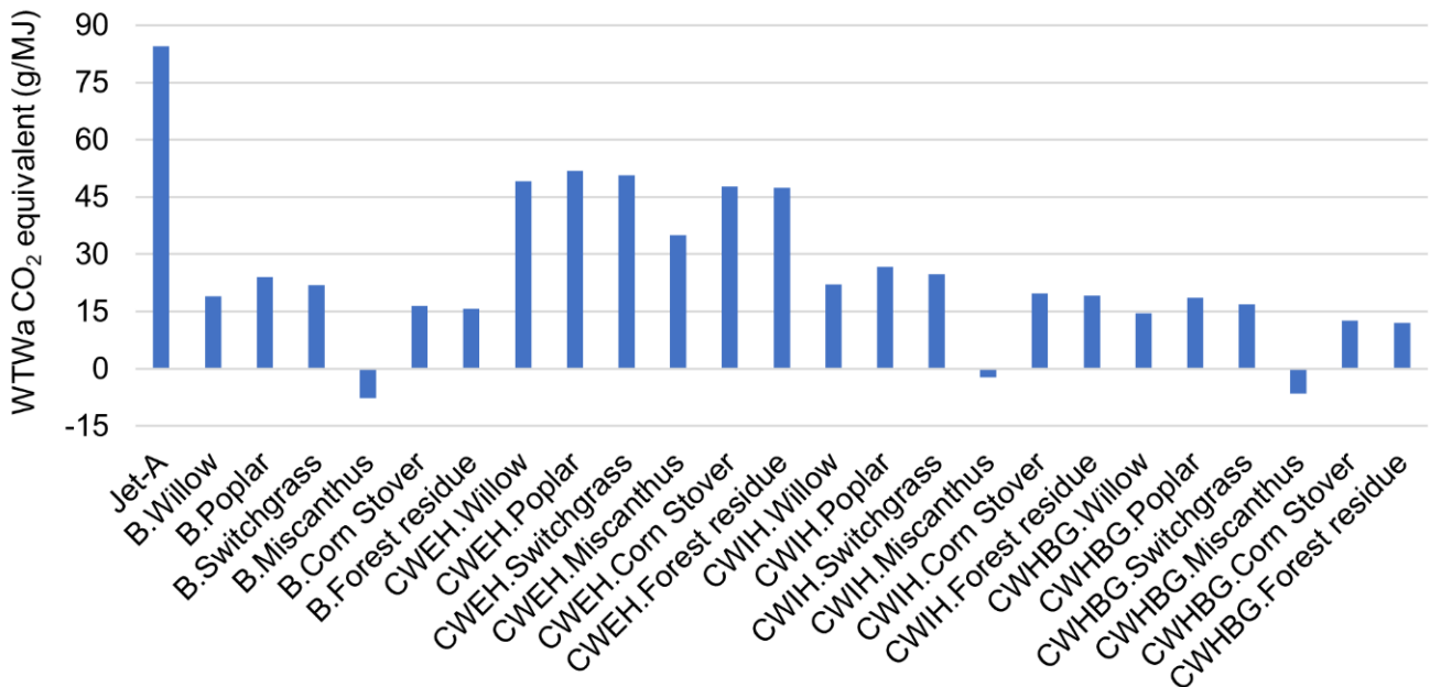
Figure 6. WTWa CO 2 equivalent emission comparison of different STJ feedstocks for 2020 (with only CO 2 emissions in PTWa phase)
