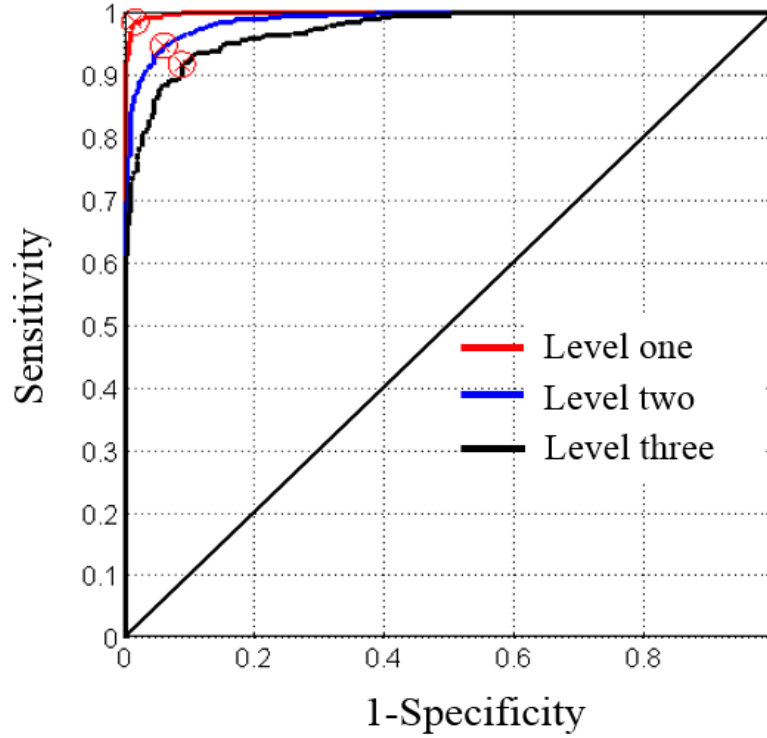
Fig 6. ROC curves of multiclass SVM with ECOC. The red circles at the upper left corner represent the cut-off points.
