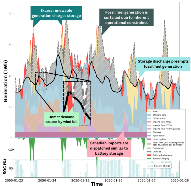
Figure 5: Winter wind lull and peak annual demand GEM results for pathway B1 (Simulation #1, 23 rd to 28 th January 2050).
