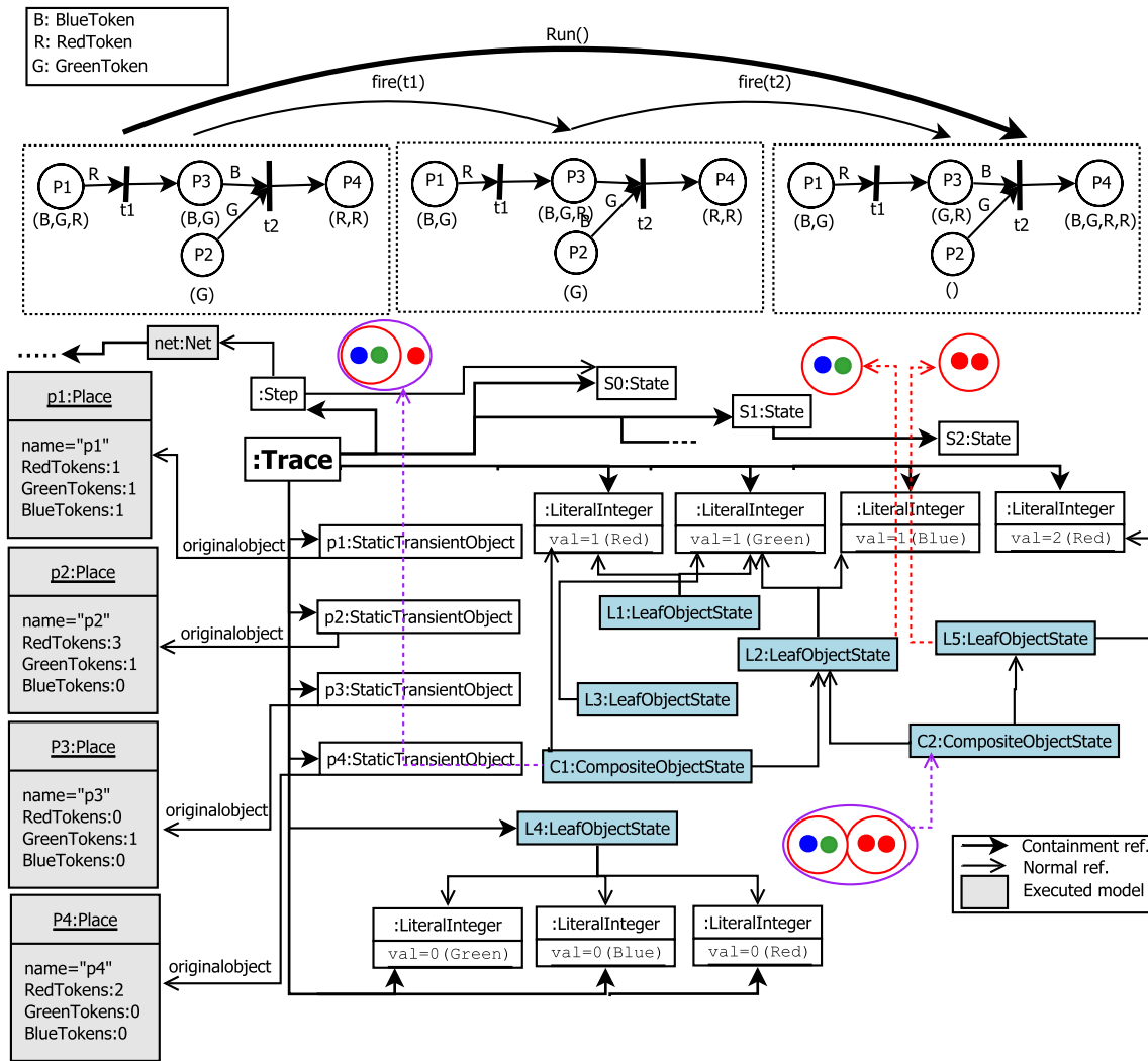
Fig. 12 Excerpt of an execution trace of the colored Petri net example model ( ObjectState with compaction) (color figure online)
