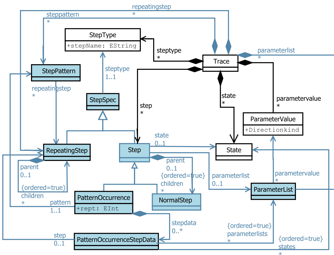
Fig. 8 Excerpt of CTM with modeling concepts related to Step , with the changes highlighted in blue (color figure online)
