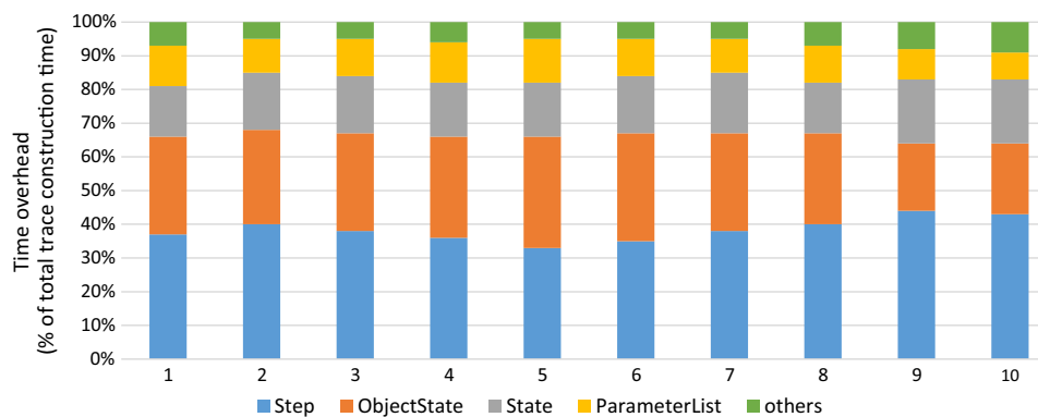
Fig. 18 Runtime overhead of the CTM and domain-specific trace construction, for each executed model
