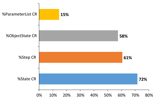
Fig. 17 Compaction rate of CTM trace elements
