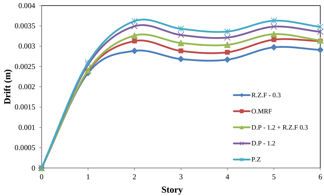
Fig. 9 Drift results of 6 story frame (R.Z.F. = 0.3, D.P. = 1.2)
