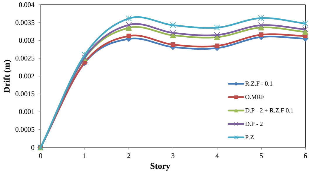
Fig. 13 Drift results of 6 story frame (R.Z.F. = 0.1, D.P. = 2.0)
