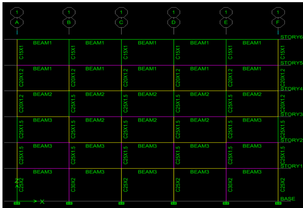
Fig. 2 Typical beams and columns in 6 stories frames
