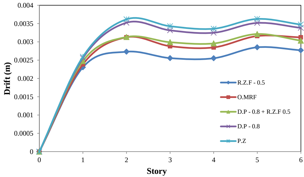
Fig. 5 Drift results of 6 story frame (R.Z.F. = 0.5, D.P. = 0.8)
