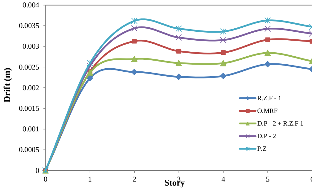
Fig. 17 Drift results of 6 story frame (R.Z.F. = 1.0, D.P. = 2.0)
