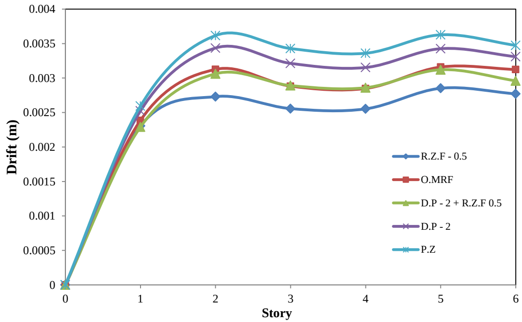
Fig. 15 Drift results of 6 story frame (R.Z.F. = 0.5, D.P. = 2.0)
