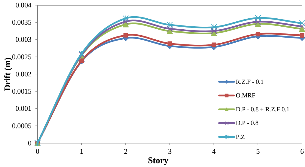
Fig. 3 Drift results of 6 story frame (R.Z.F. = 0.1, D.P. = 0.8)
