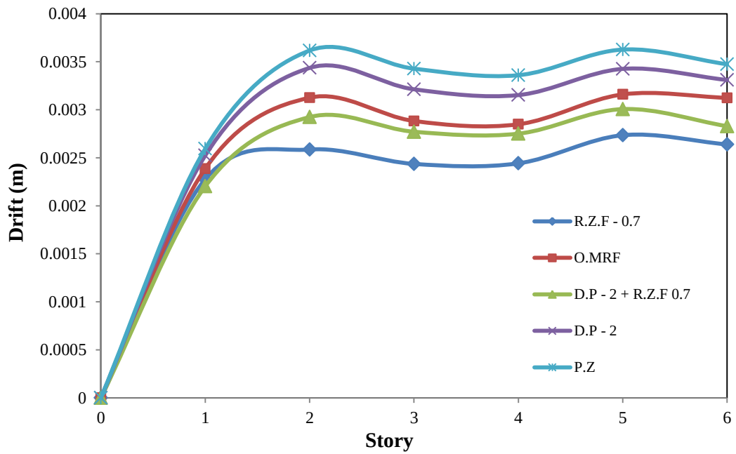
Fig. 16 Drift results of 6 story frame (R.Z.F. = 0.7, D.P. = 2.0)
