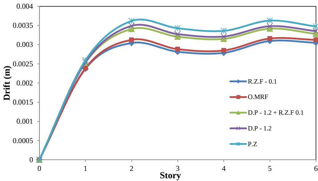
Fig. 8 Drift results of 6 story frame (R.Z.F. = 0.1, D.P. = 1.2)
