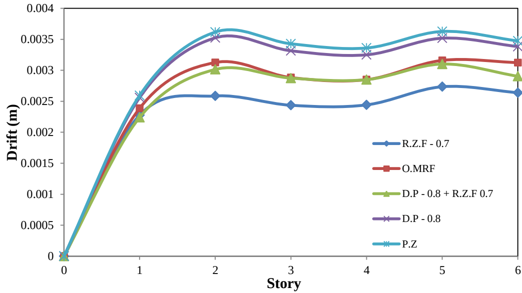
Fig. 6 Drift results of 6 story frame (R.Z.F. = 0.7, D.P. = 0.8)
