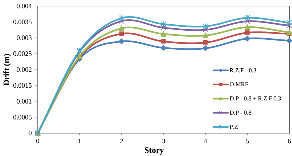
Fig. 4 Drift results of 6 story frame (R.Z.F. = 0.3, D.P. = 0.8)
