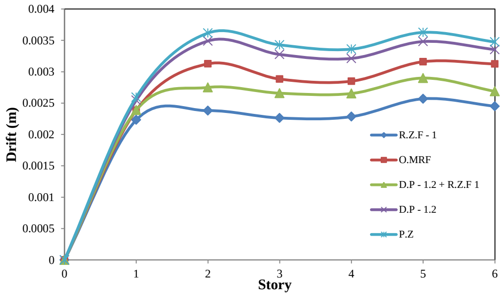
Fig. 12 Drift results of 6 story frame (R.Z.F. = 1.0, D.P. = 1.2)
