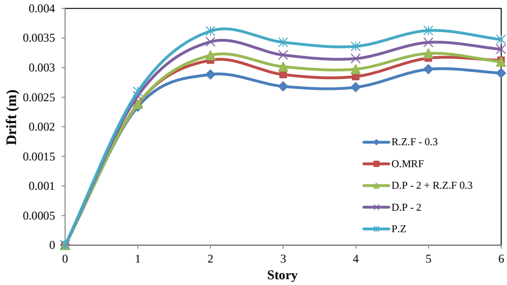
Fig. 14 Drift results of 6 story frame (R.Z.F. = 0.3, D.P. = 2.0)
