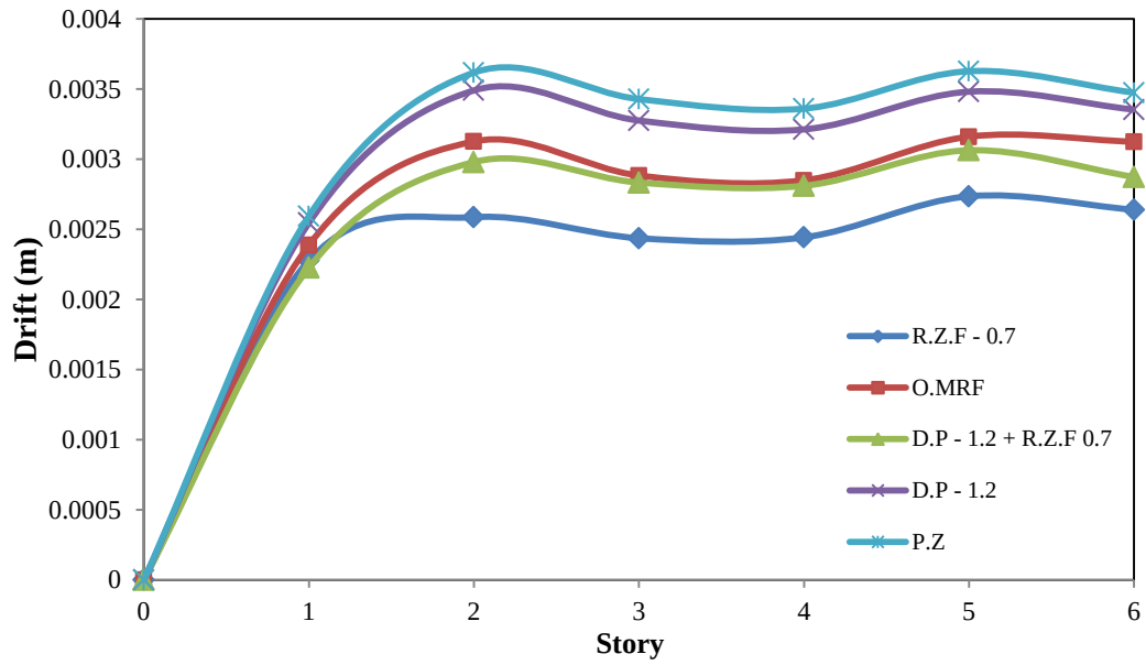
Fig. 11 Drift results of 6 story frame (R.Z.F. = 0.7, D.P. = 1.2)
