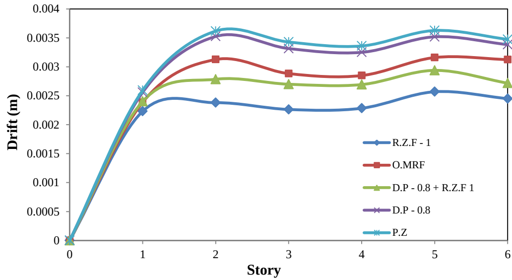
Fig. 7 Drift results of 6 story frame (R.Z.F. = 1.0, D.P. = 0.8)
