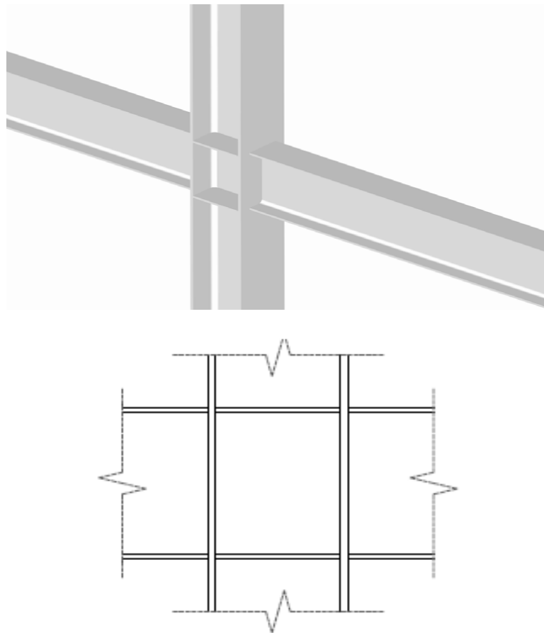
Fig. 1 Illustration of the panel zone, as illustrated by Davila-Arbona (2007)
