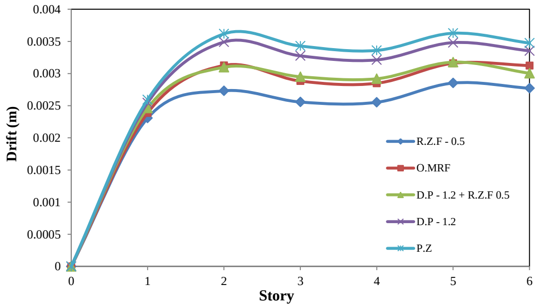
Fig. 10 Drift results of 6 story frame (R.Z.F. = 0.5, D.P. = 1.2)
