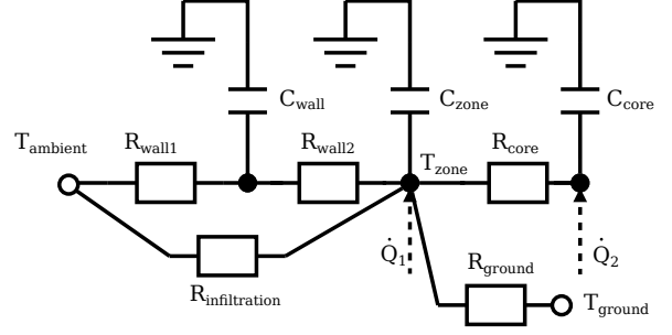
Figure 2: 5R3C building model
