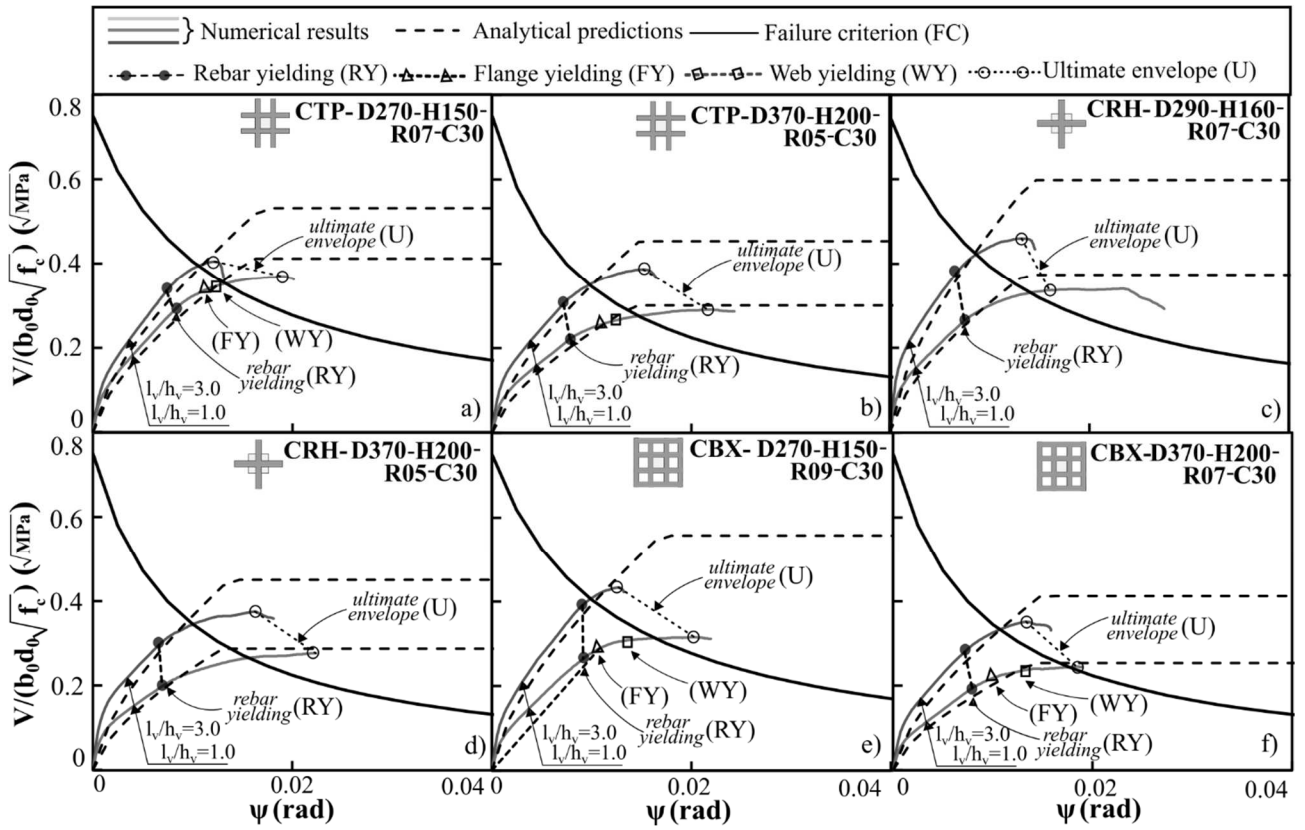
Figure 11 Influence of the slab radius on the slab capacity and rotations a) CTP, d=270 mm, h_v=150 mm, \rho_l=0.7\% f_c=30 MPa; b) CTP, d=370 mm, h_v=200 mm, \rho_l=0.5\% f_c=30 MPa; c) CRH, d=290 mm, h_v=160 mm, \rho_l=0.7\% , f_c=30 MPa; d) CRH, d=370 mm, h_v=200 mm, \rho_l=0.5\% , f_c=30 MPa; e) CBX, d=270 mm, h_v=150 mm, \rho_l=0.9\% f_c=30 MPa; f) CBX, d=370 mm, h_v=200 mm, \rho_l=0.7\% f_c=30 MPa
