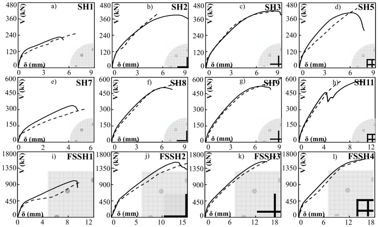
Figure 6 Numerical validations: Chana & Birjandi (1996) test series [20] a) SH1, b) SH2, c) SH3, d) SH5, e) SH7, f) SH8, g) SH9, h) SH11, i) FSSH1, j) FSSH2, k) FSSH3, l) FSSH4; (continuous black curves represent the V - \delta from numerical simulations, whilst dashed black curves depict V - \delta from tests)
