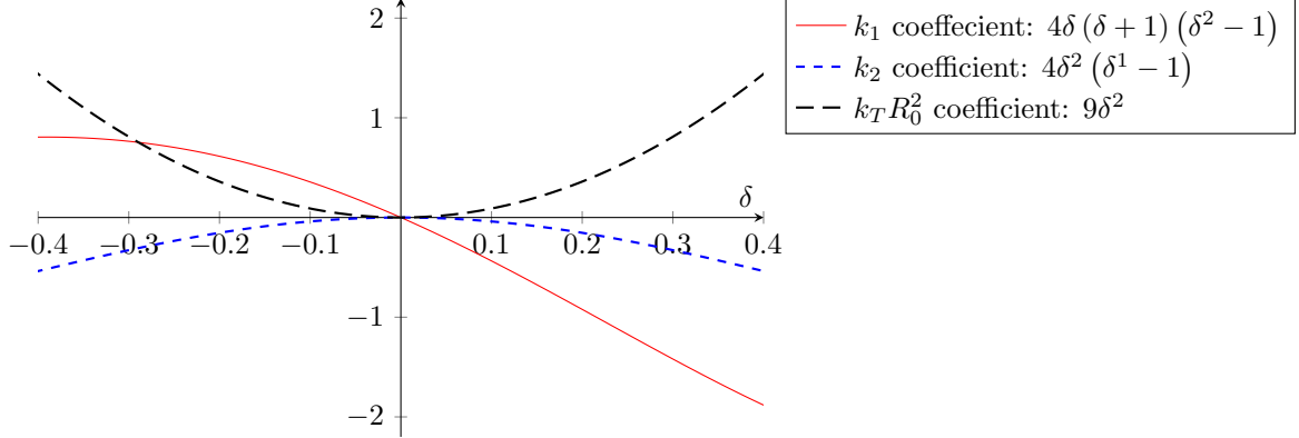
Figure 13: Effect of \delta on the three terms forming the restoring torque nonlinearity
