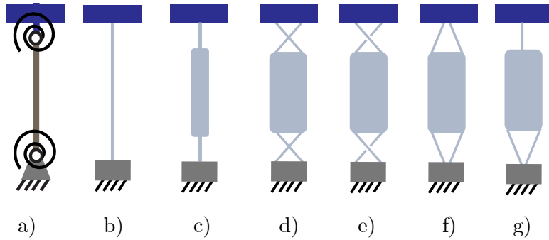
Figure 9: Flexure equivalents for the connecting rods
