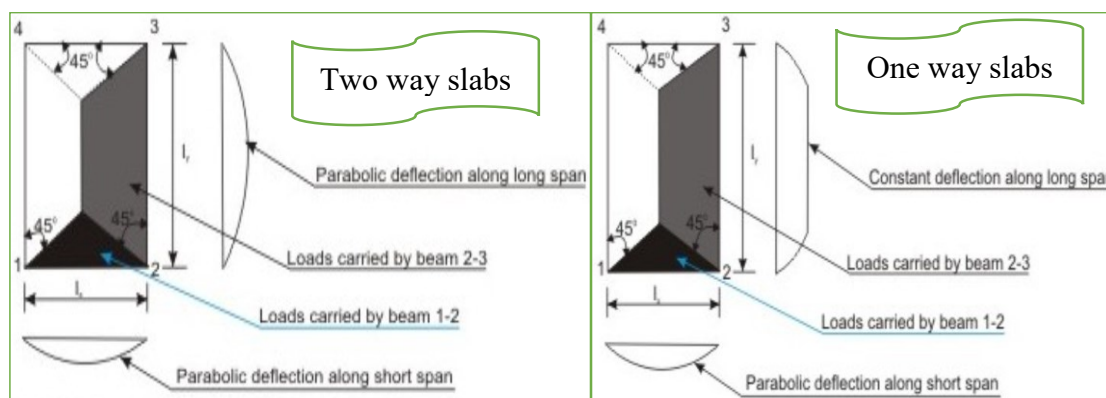
Figure 2.37 Two-Way and One-Way Slab Load Sharing.
