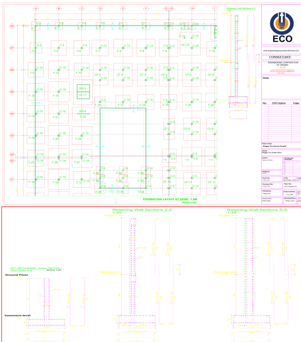
Figure 2.32 Retaining Wall Section Detail and Layout within Foundation of MHB
