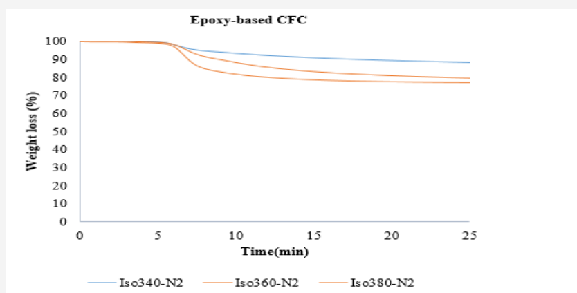
Figure 1: Isothermal TGA curve of epoxy-based CFC recorded in nitrogen (considering the influence of temperature).
