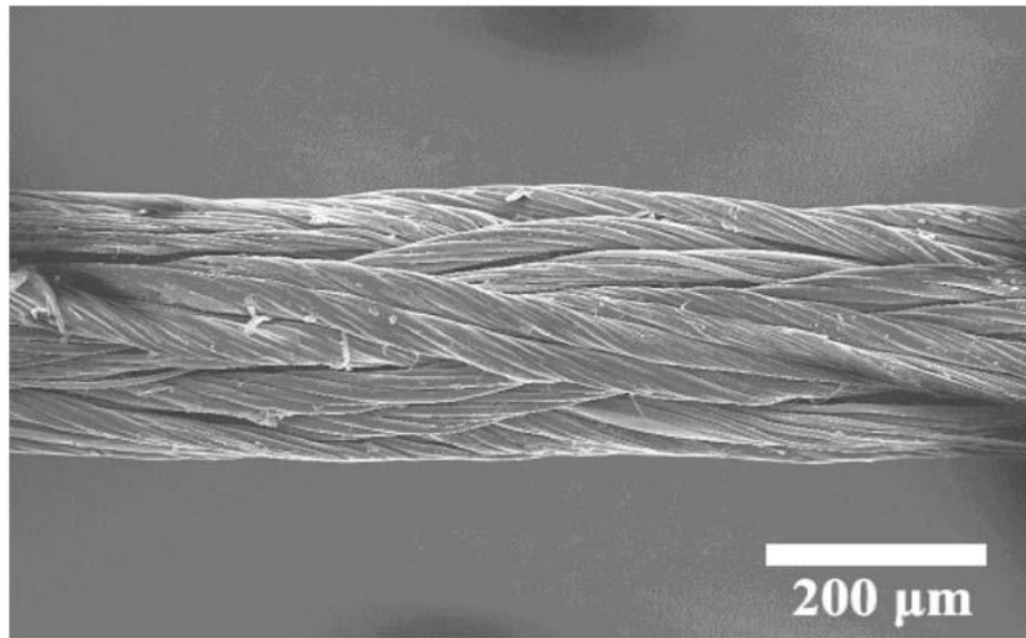
Figure 1. SEM image of a carbon nanorope 13 .
