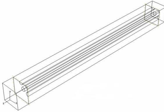
Figure 2. The RVE used to simulate the CNT bundle-reinforced polymer.
