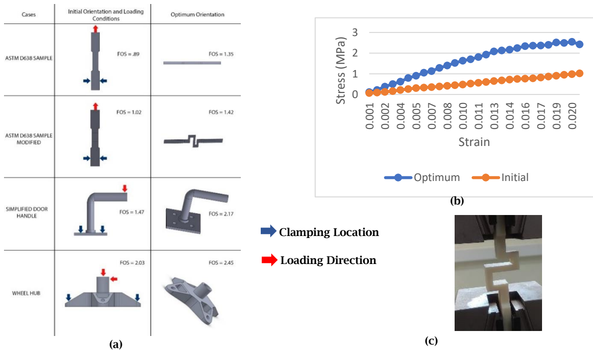
Fig. 5: (a) Computational Experiments (b) Experimental Results (c) Custom design object on UTM.
