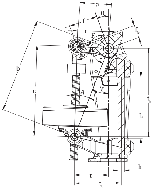
Fig. 2. Linkage geometry labels. The optimization procedure searched for the t, t_k, f, f_k, L geometry parameters. The objective was finding moment arm geometry with the most efficient configuration of the power stroke as specified by the load trajectory and actuator dynamics.
