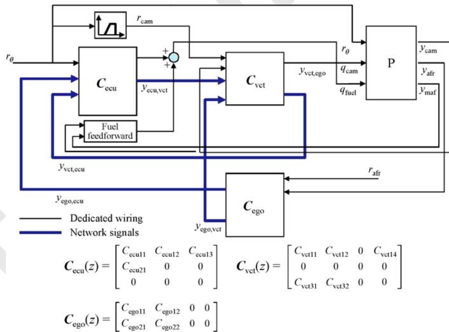
Fig. 7 Controller distribution to maximize VCT actuator modularity
