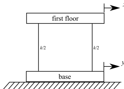
Figure 3.31: A 1-DOF latterly excited system that represents a 1-story building.
