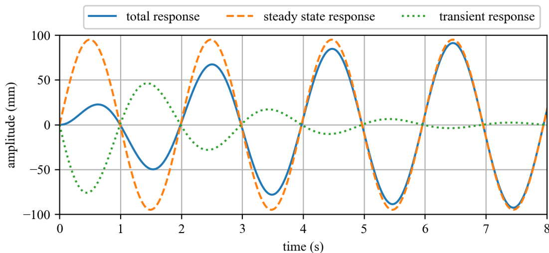
Figure 3.16: Temporal responses for a underdamped system with k = 100 N/m, m = 10 kg, c = 10 kg/s, F_0 = 3 N, and \omega = 3.162 .
