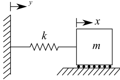
Figure 3.32: A base excited 1-DOF spring-mass system.
