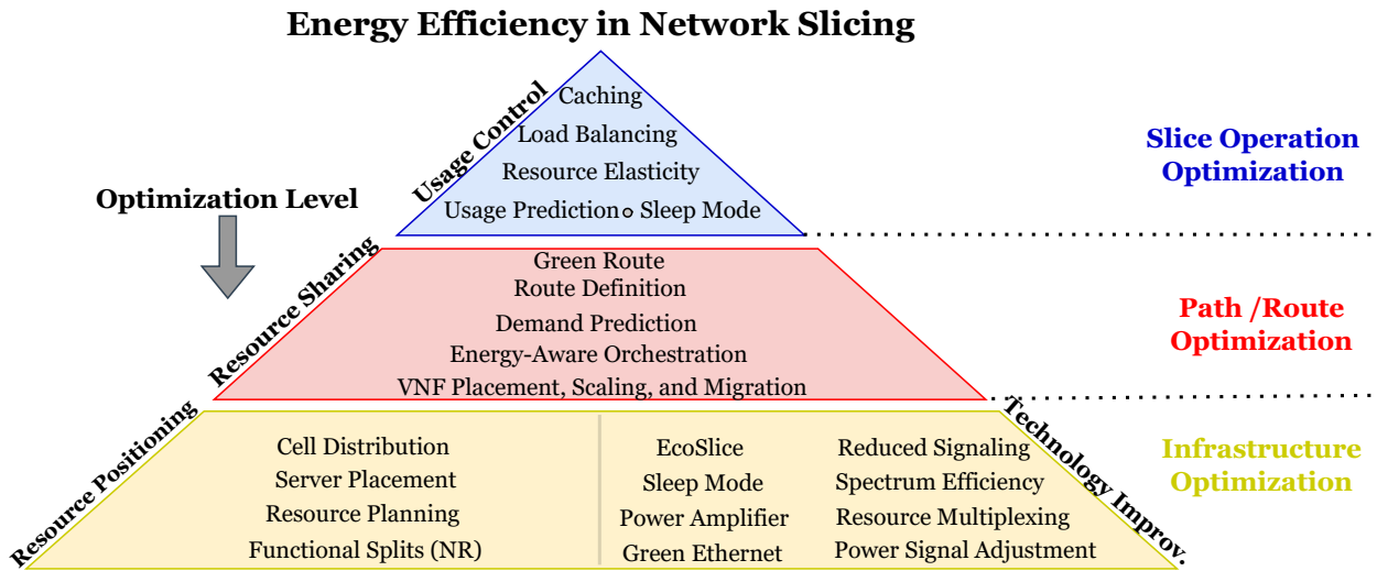
FIGURE 5. Optimization levels to increase energy efficiency in Network Slicing.
