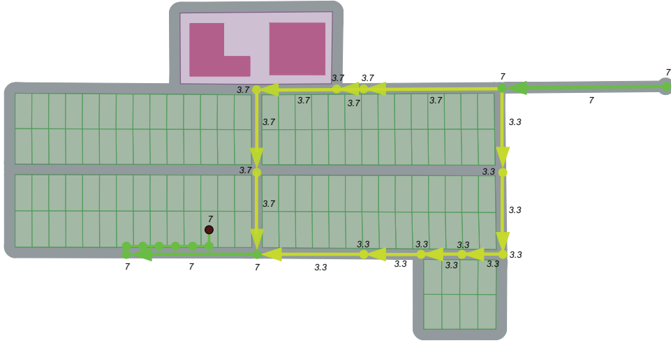
Fig. 2. Calculation of expected amount of flow delivered from source (green) to a demand node (black). Nodes/links that do not supply resources to the demand node are not shown.
