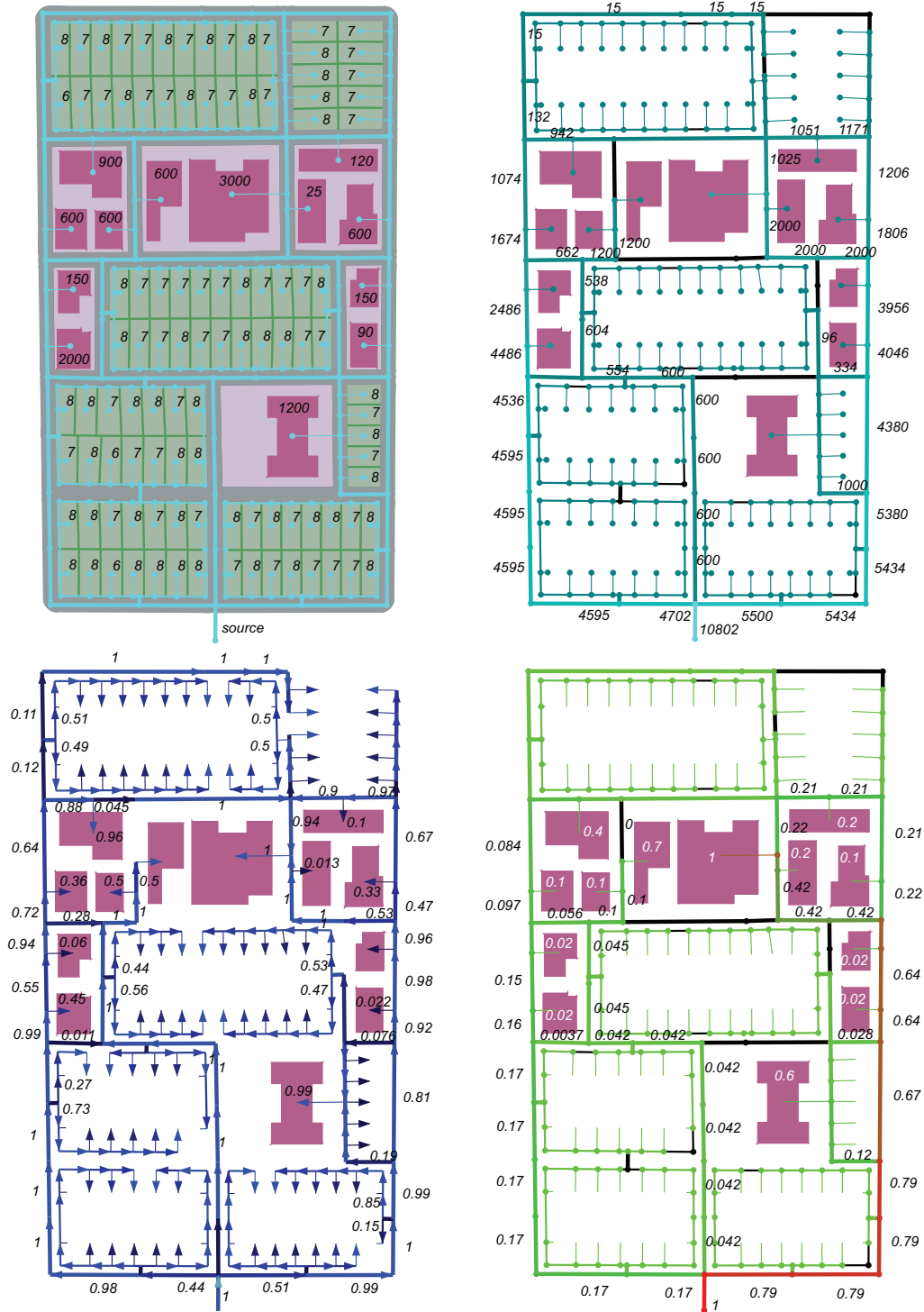
Fig. 3. Four steps in critical flow computation. Upper left: network topology with demands. Upper right: maximum flow. Lower left: induced probability graph. Lower right: critical flow (CFC), with light green being non-critical and red being critical.
