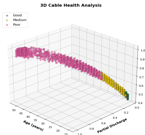
Figure 7. 3D relationships among cable age, discharge, and corrosion.
