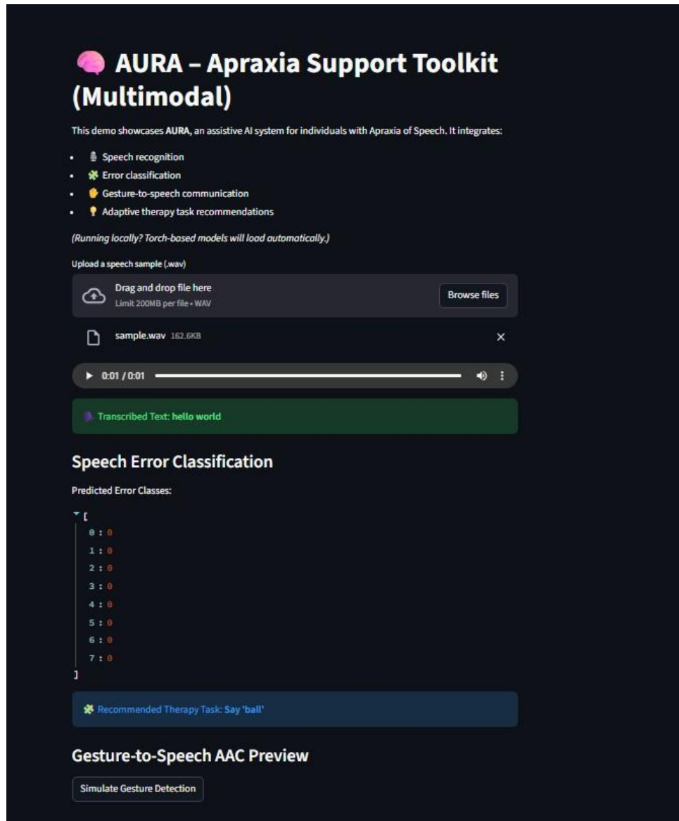
Fig 4: AURA prototype interface showing the speech-based demo workflow and an exploratory gesture-based AAC module presented as an optional extension.
