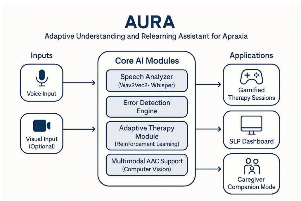
Fig 1: AURA system architecture showing the input layer (voice and optional visual input), core AI processing modules (speech analysis, error detection, adaptive therapy, and multimodal AAC), and user-facing applications including gamified therapy, clinician dashboard, and caregiver companion tools.
