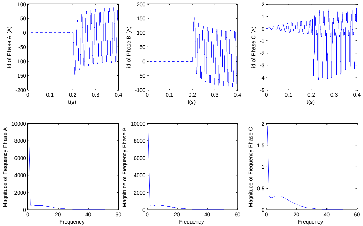
Figure 11: Differential Currents and Frequency Range obtained of Output of S transform related to two-phase internal error due to change in residual flux
