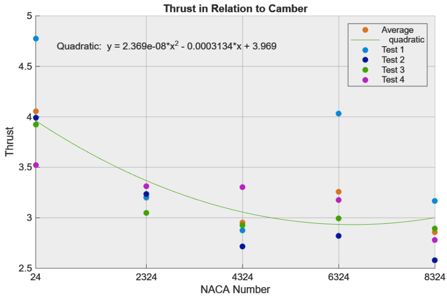
Figure 7: MATLAB graph of camber data.
