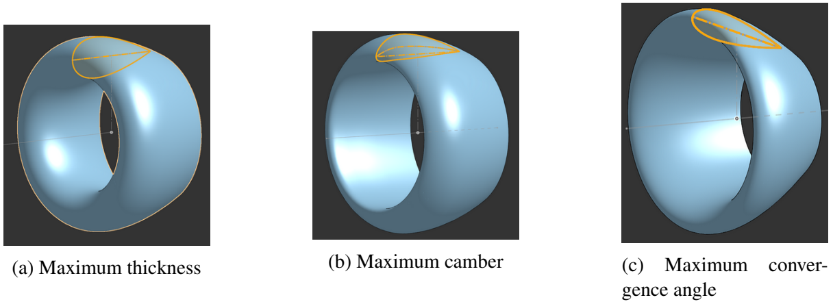
Figure 2: Visualization of maximum collector electrode geometries
