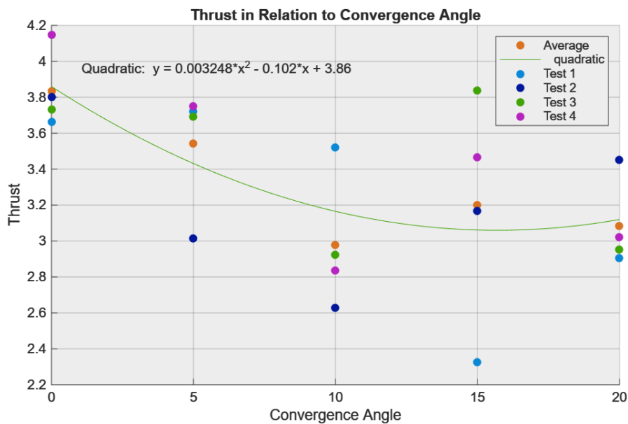
Figure 8: MATLAB graph of convergence angle data.
