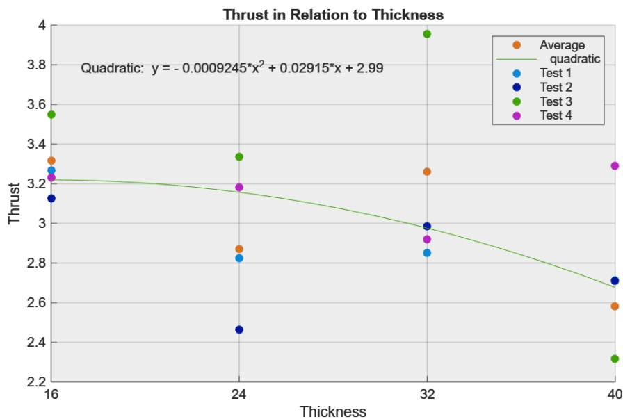
Figure 6: MATLAB graph of thickness data.
