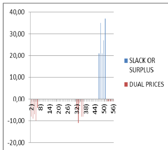
Figure 2: Graph of slack or surplus
