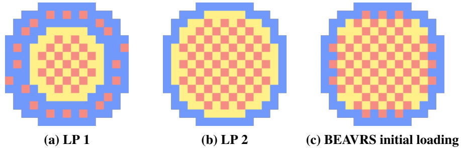
Figure 4: LP designs using SQA for a three fuel-type PWR compared with the initial core LP in the BEAVRS benchmark [7].
