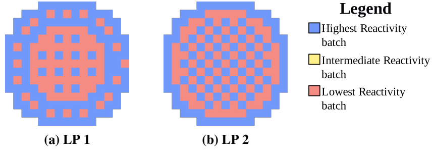
Figure 3: LP designs using SQA for a two fuel-type PWR.
