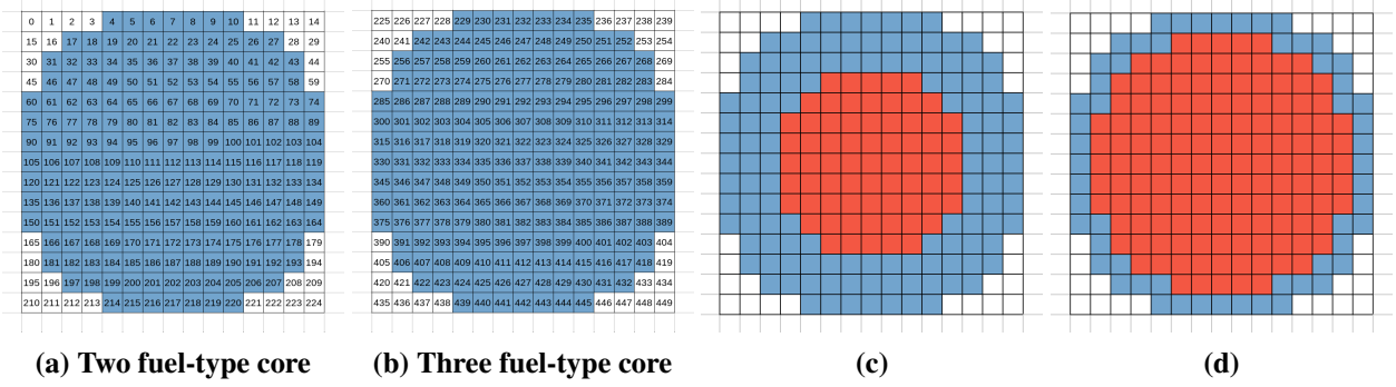
Figure 1: Core representation with qubits on a regular grid (a, b) and examples of transverse fields, h , defining inner and outer regions (c, d).
