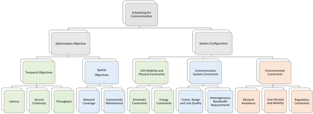
Fig. 9. Structure of Section 6. Scheduling for communication.
