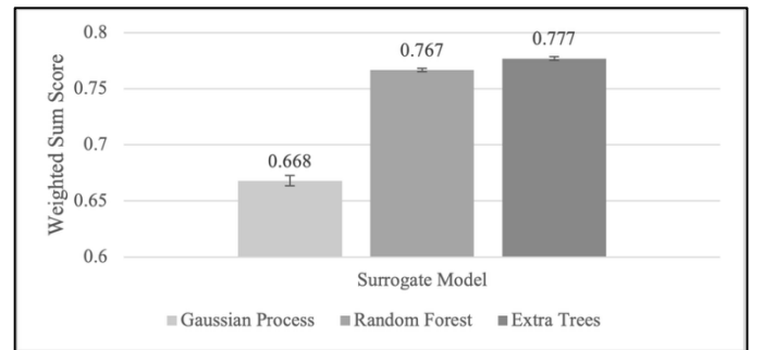
Figure 3. The Effect of Different Surrogate Models on Weighted Sum Score
