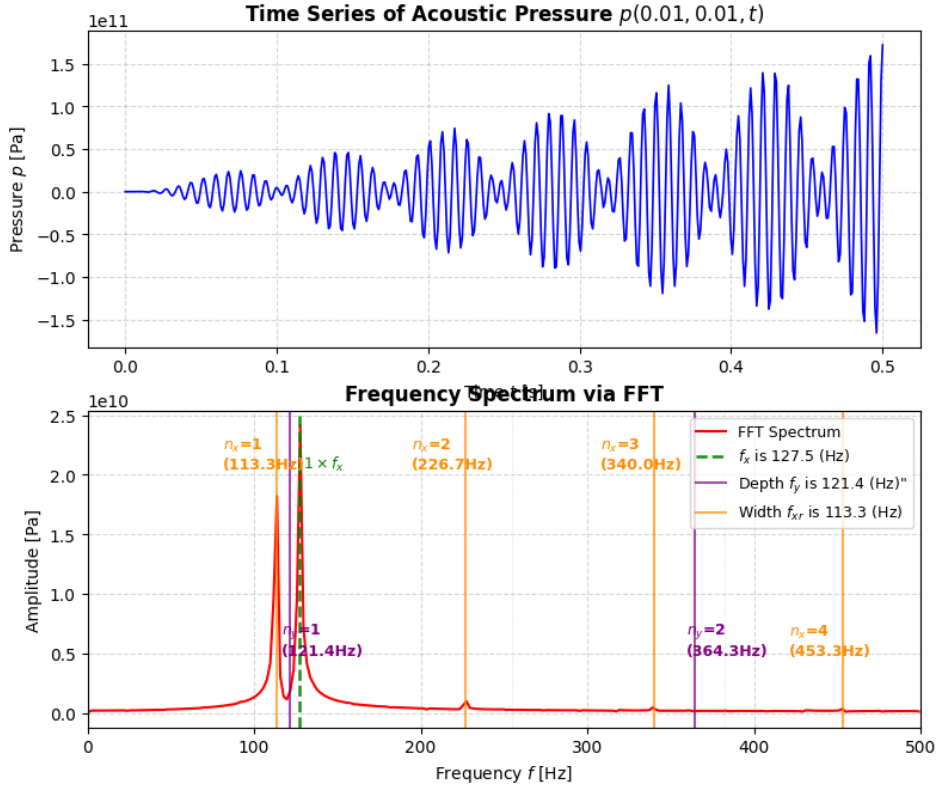
Fig. 5 Numerical Calculation Result ( U = 1700.0(\text{m/s}) )
