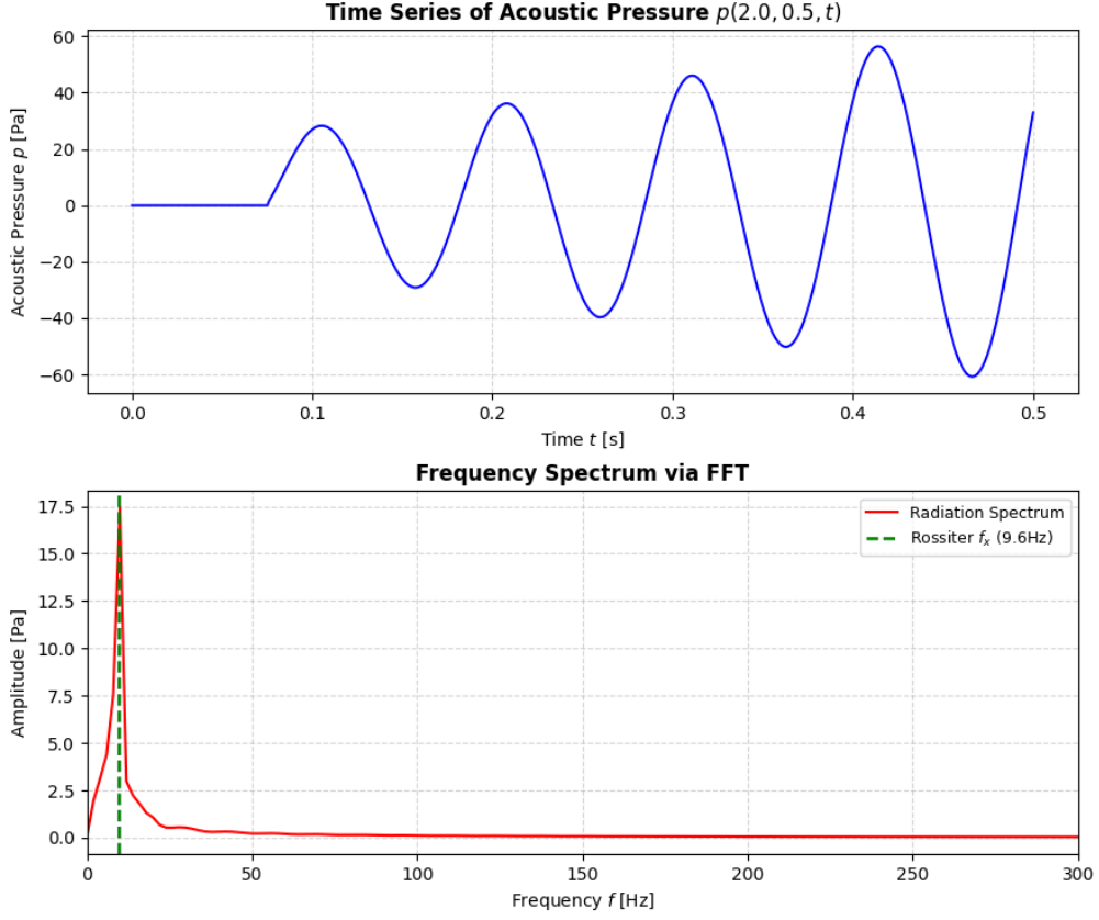
Fig. 3 Numerical Calculation Result ((x,y) = (2.0,0.5))
