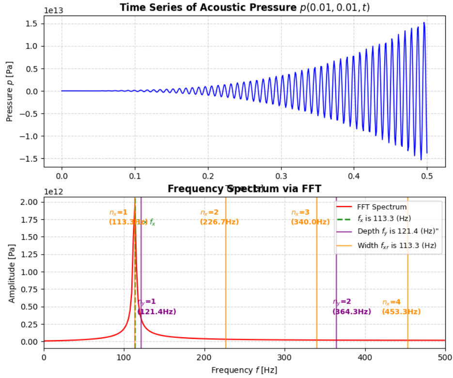
Fig. 4 Numerical Calculation Result ( U = 1133.3(\text{m/s}) )
