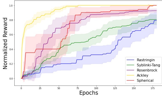
Figure 5: Validation of MixMOBO on five standard benchmark functions. Mean normalized reward is plotted with shaded regions representing 0.5\times standard deviation [20].
