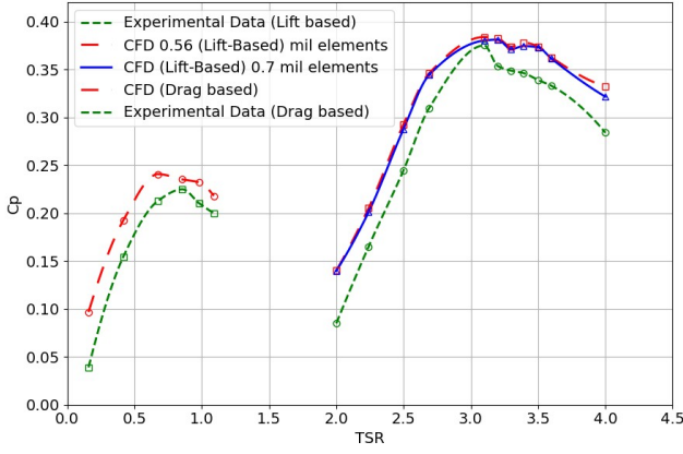
Figure 4: Validation of Savonius (Drag-based) with Blackwell et al. [28] and Darrieus (Lift-based) turbines with Bachant and Wosnik [26].
