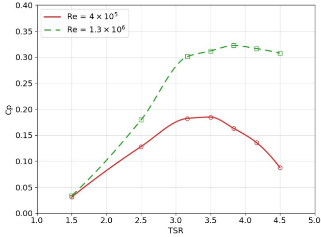
Figure 16: Comparison of Reynolds number for the benchmark Darrieus turbine at Re = 4 \times 10^5 (circles with solid line) and Re = 1.3 \times 10^6 (squares with dashed line).
