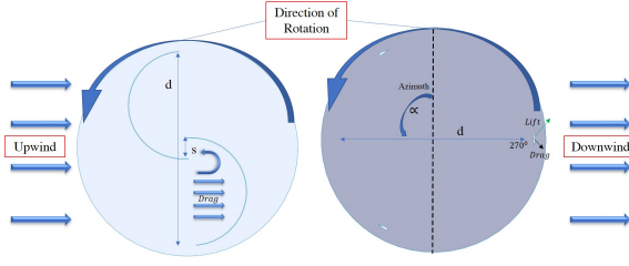
Figure 13: Schematic for (a) Savonius and (b) Darrieus turbines
