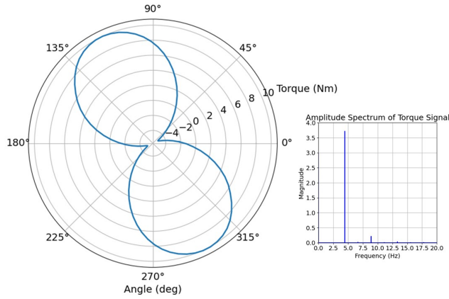
Figure 7: Torque versus azimuth and corresponding FFT for the best VAWT design
