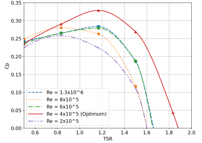
Figure 11: Comparison of C_p as a function of TSR for the optimized VAWT blade across different Re .
