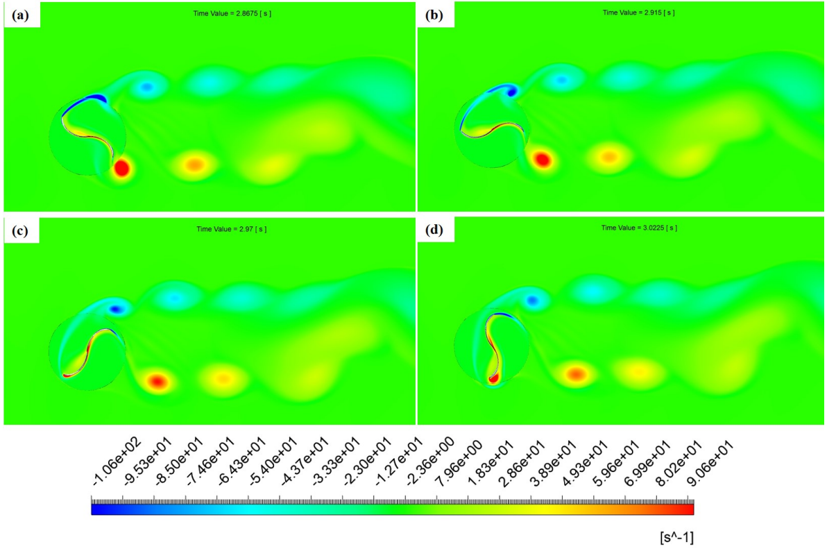
Figure 8: Vorticity contours for the optimum shape at (a) T/8 , (b) T/4 , (c) 3T/8 , and (d) T/2 . Contours are symmetric from T/2 to T .
