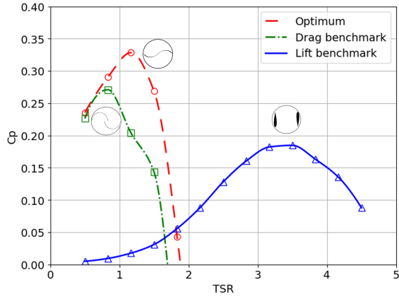
Figure 9: Comparison of benchmark drag-based ( s/d = 0.2 ) and lift-based (scaled for visualization) configurations with optimum (Best design).
