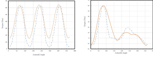
Figure 15: Overall (left) and blade torque (right) comparison with respect to azimuth angle for the present CFD results (solid line) and CFD results from Siddique et al. [31] (dashed line).
