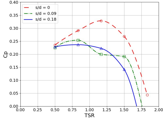
Figure 10: Comparison of overlap ratios of 0, 0.09, and 0.18 for optimum blade shape.
