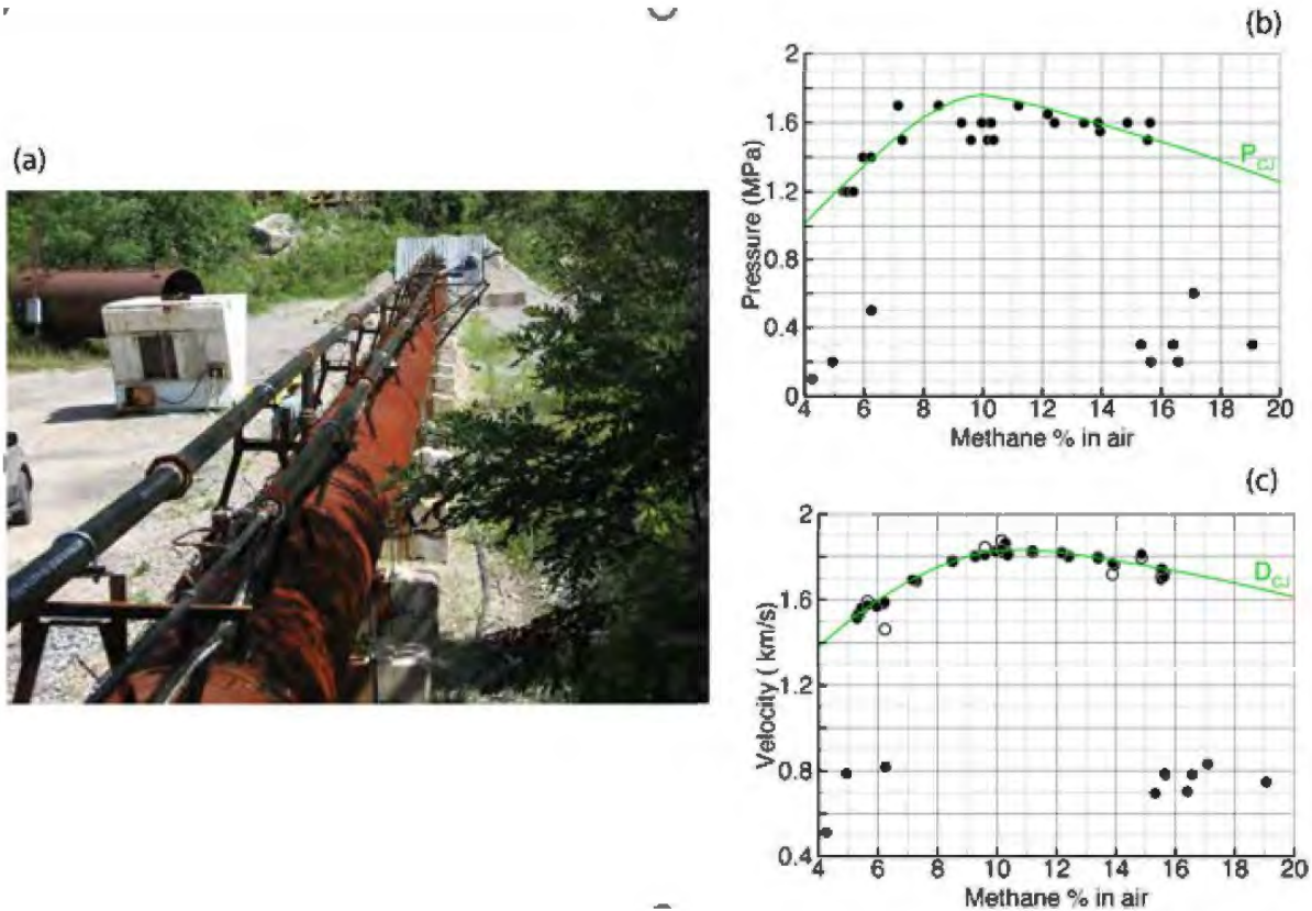
Figure 2.7 (a) The Gas Explosion Text Facility ( GETF) at Lake Lynn Experimental Mines, showing the 72 m long, 1-m-diameter shock tube used for methane-air detonability studies. (b) and (c) Data obtained for front velocity and pressure behind the shock wave as a function of the stoichiometry in the channel. Black points are data, green lines marked P_{CJ} and D_{CJ} are theoretical values of pressure and detonation velocity. Details of experiment and interpretation of the data are given in [19]. Note that the fall-offs in the values of velocity and pressure at high and low values of % of methane indicate the detonability limit, which is not predicted by theory.
