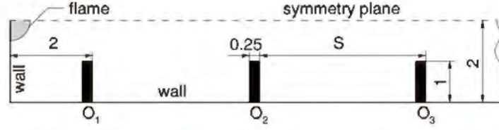
Figure 2.1 Schematic of computational domain.
