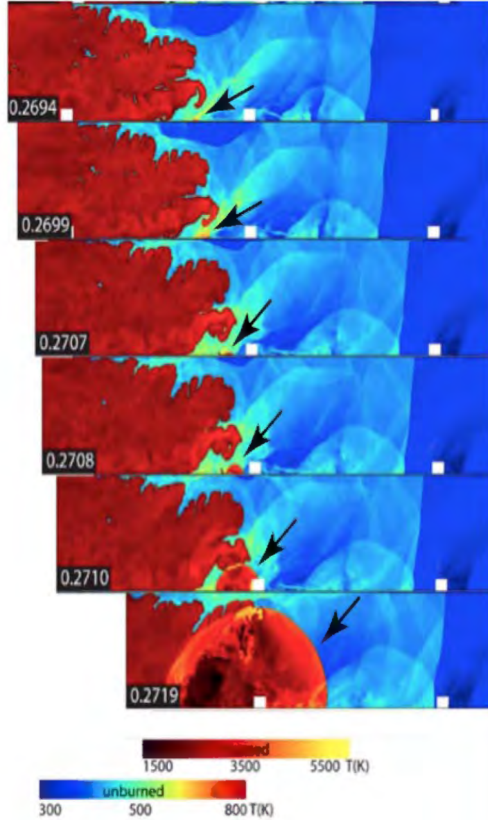
Figure 2.9 Simulation showing the transition to detonation in an obstacle-laden channel filled with a fuel-air mixture and for low blockage in the system. The obstacles are indicated by the small white squares on the bottom wall. The mechanism for transition in this case is multiple shock collisions leading to energy focusing at a location near the lower boundary. The arrows point to the location of detonation ignition. Details are given in [11, 12].
