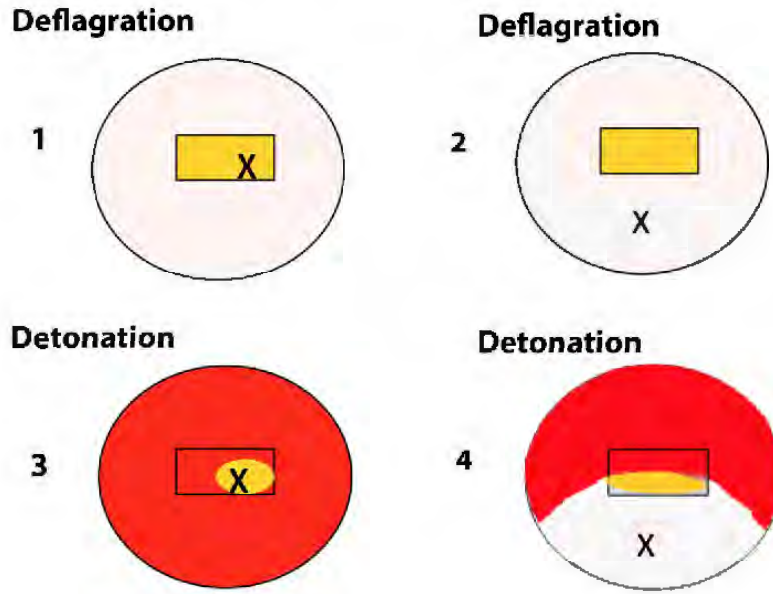
Figure 3.2 Four VCE scenarios. The ovals represent a top view of a pancake-shaped flammable cloud, the rectangles are congested regions of industrial plants and X marks the ignition point. Red indicates detonation regions, pink indicates the cloud fire, and yellow indicates a deflagration.
