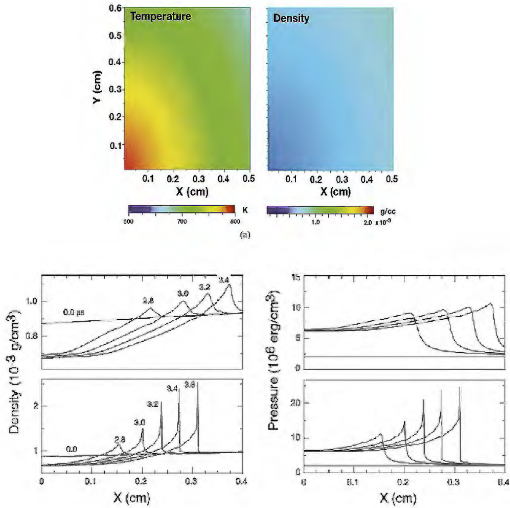
Figure 2.4 Evolution of a gradient in reactivity [15]. Top figure: Maps of the initial temperature and density, with pressure held constant. Bottom figure: Profiles showing the evolution of density and pressure for the vertical and horizontal directions. Top row: The shallower gradient never becomes a detonation before leaving the hot spot. Instead, it decays into a shock with a flame left behind it. Bottom row: A spontaneous wave shows transition to a shock and detonation inside the hot spot. Times in \mu s.
