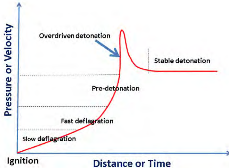
Figure 1.1 Schematic showing the phases in the evolution of a combustion system from a deflagration to a detonation.
