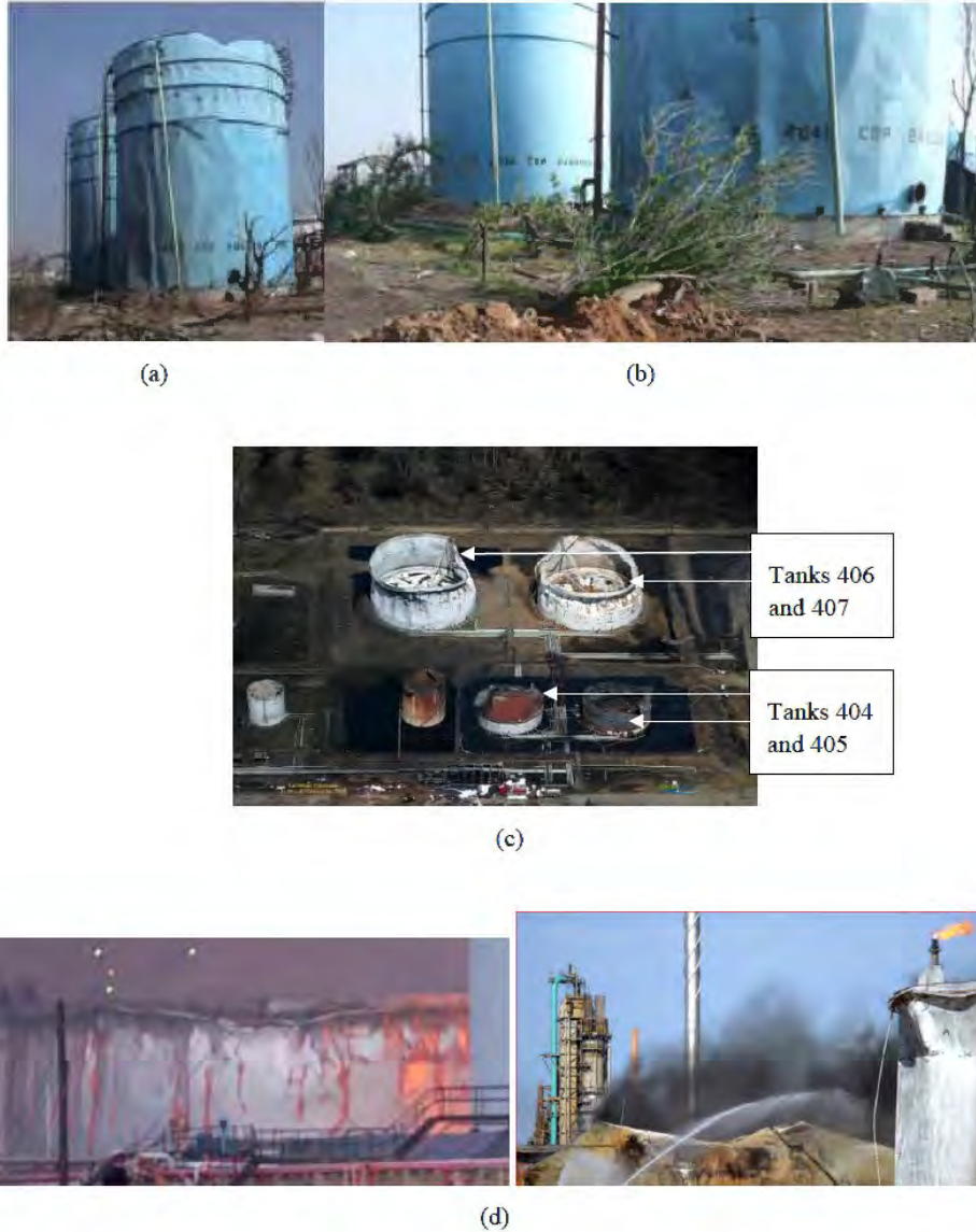
Figure 4.8 Views of a crushed, empty firewater tank at Jaipur (a) from a distance and (b) close by [4]. Empty tanks at (c) Puerto Rico [49, 38] (reproduced by permission of the Fire and Blast Information Group, (FABIG), www.fabig.com ) and (d) Amuay [50].
