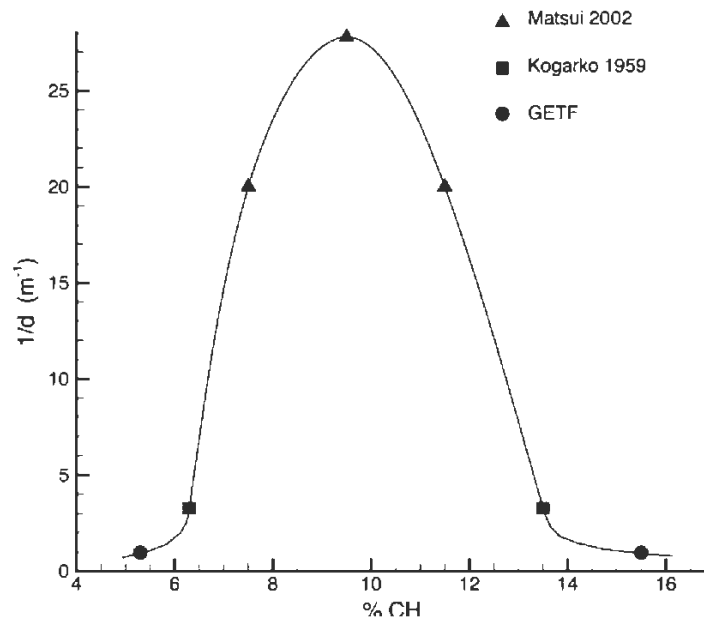
Figure 2.8 Comparison of GETF detonability limits to measurements in smaller diameter channels as a function of 1/d , the inverse of the diameter of the channel. The limits expand with the size of the channel [19].
