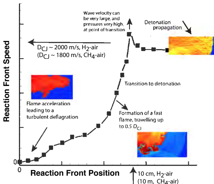
Figure 2.3 The details of Figure 2.2 related to the stages of flame acceleration and DDT shown in Figure 1.1. Figure is marked for both hydrogen-air in a small, 4-cm channel [22] and, in parentheses on the axes, for methane-air in 17-cm channel [24].
