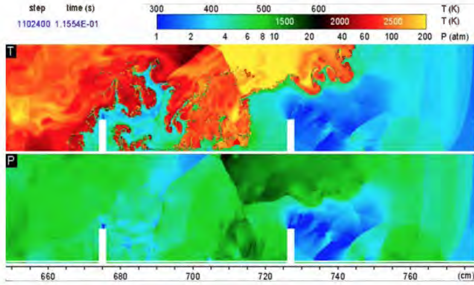
Figure 2.6 One time in a simulation of a turbulent deflagration propagating in an obstacle-laden channel containing a stoichiometric mixture of methane and air initially at atmospheric conditions. Top frame is temperature and bottom frame is pressure. Color bars across the top show two temperature scales, the upper for unburned fuel and the lower for burned fuel. The turbulent, unreacted flow contains many shocks in both the fuel and product. Many of these, especially those generated at the flame surface, propagate forward and strengthen the leading shock (on the far right). Other shocks interacting with the flame front wrinkle the front more through shock-flame interactions. This is discussed further in [24].
