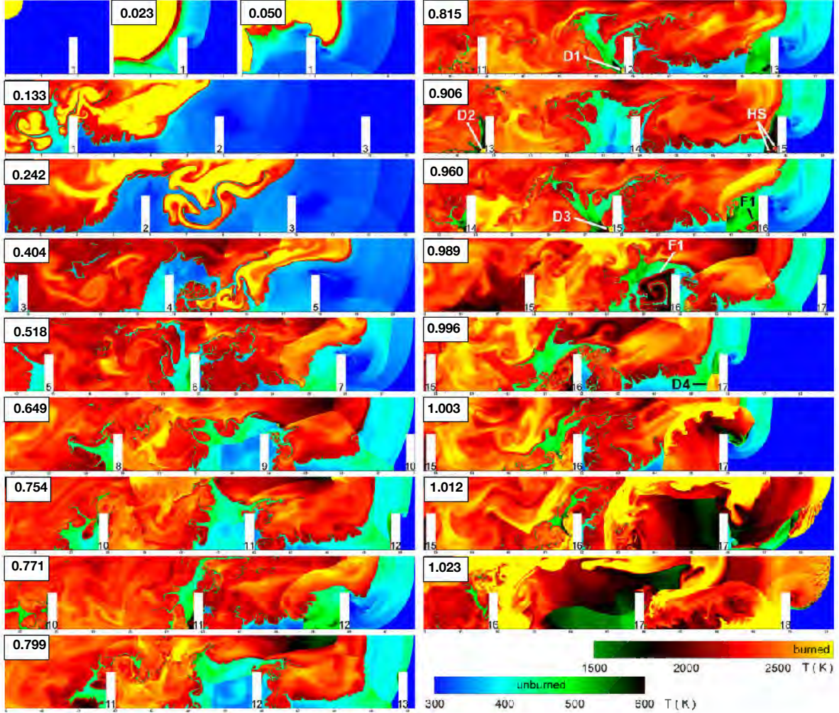
Figure 2.2 Results from a numerical simulation showing the transition from a small spark, to a turbulent flame, to a fast deflagration, and finally transition to a detonation, which propagates through the system [22]. This particular simulation was done for a hydrogen-air mixtures in a channel 4 cm high with obstacles 1/2 the height of the channel (blockage ratio = 0.5). Times are given in milliseconds in the upper left corner of each frame. The two temperatures scales, shown on the bottom right, are for burned and unburned material as noted. Obstacles are numbered. Symbols D1, D2, D3, D4, F1, and HS indicate hot spots (discussed in Section 2.2), failed detonations, and successful detonations (described in more detail in Sections 2.1 and 2.2). D4 indicates the hot spot that evolves into the detonation that finally dominates the combustion process in the entire channel. The simulations were obtained by solving the unsteady, two-dimensional Navier-Stokes equations with a model for chemical reactions and energy release that was calibrated to conditions produced by a stoichiometric hydrogen-air gas initially at atmospheric temperature and pressure.
