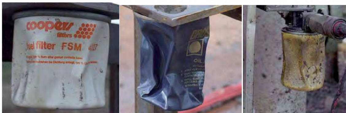
Figure 4.5 Air-filled oil filters placed inside the detonation (photograph reproduced from [32]) compared to an oil filter recovered from the Buncefield explosion (shown on the extreme right).
