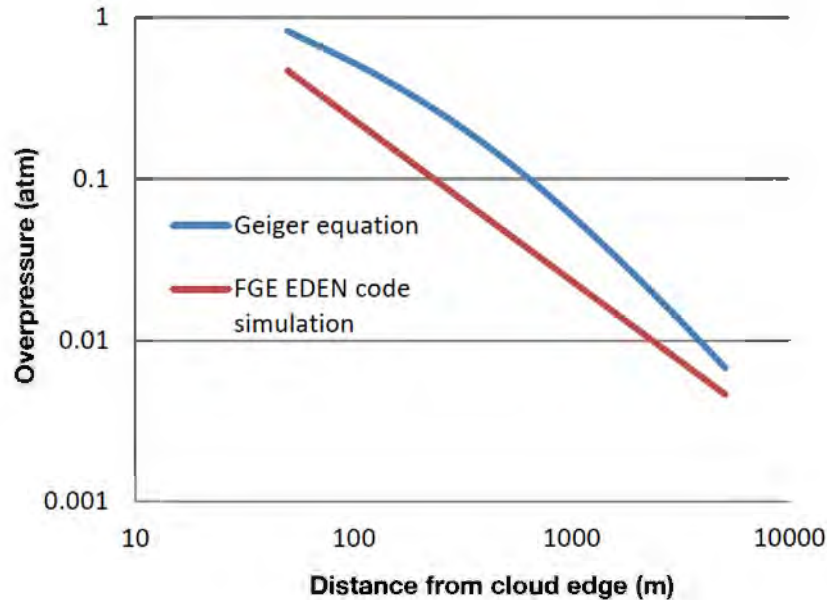
Figure 4.11 Comparison of the Geiger result (Equation (4-4), [55]) with the simplified form of a correlation based on the FGE EDEN code (Equation (4-2), [47]) for a pancake shaped cloud of radius 200 m and 3 m height.
