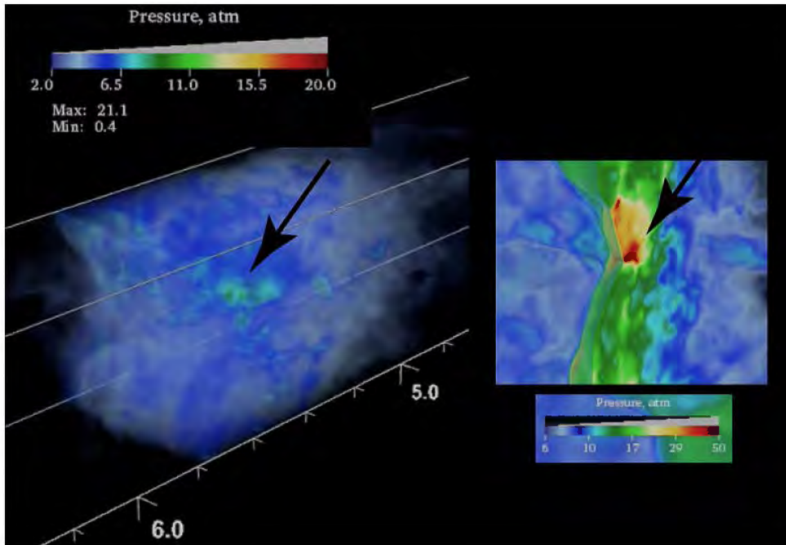
Figure 2.10 Simulation of a hydrogen-air flame embedded in a high-intensity turbulent background. Inflow-outflow boundary conditions on end walls. Periodic boundary conditions on
